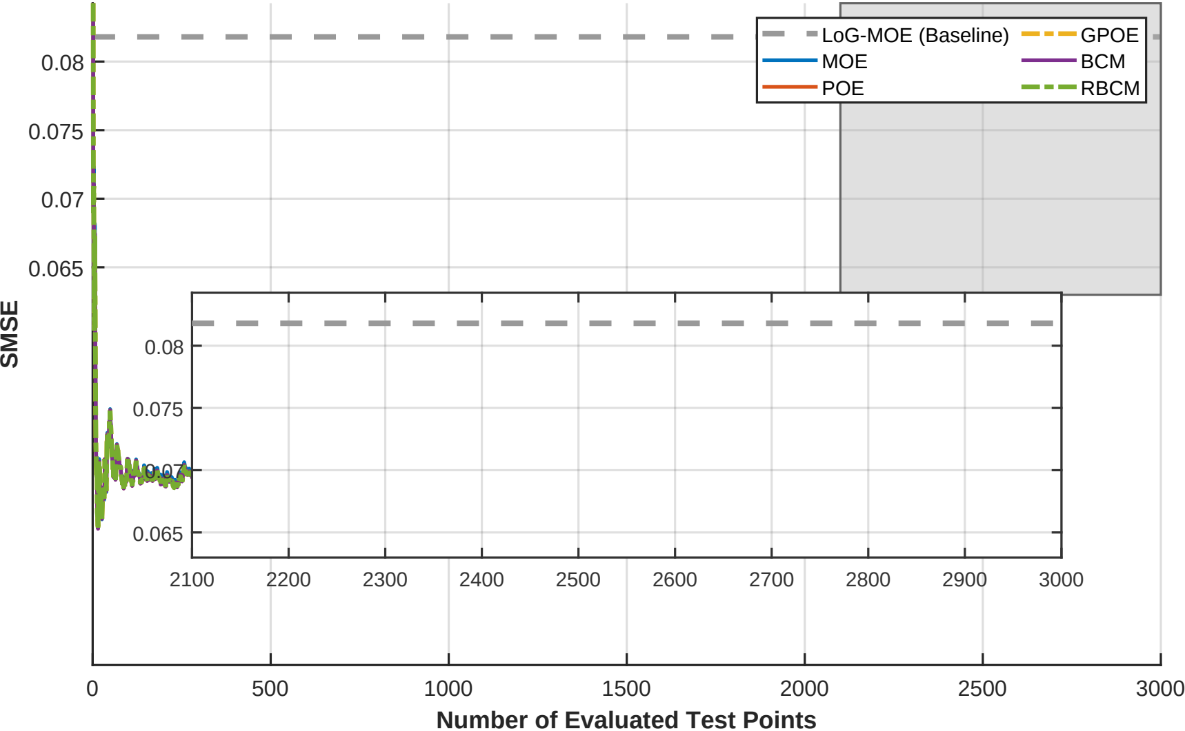
PUMADYN32NM - Fig3 TP AC - SMSE (5 MC Avg)
