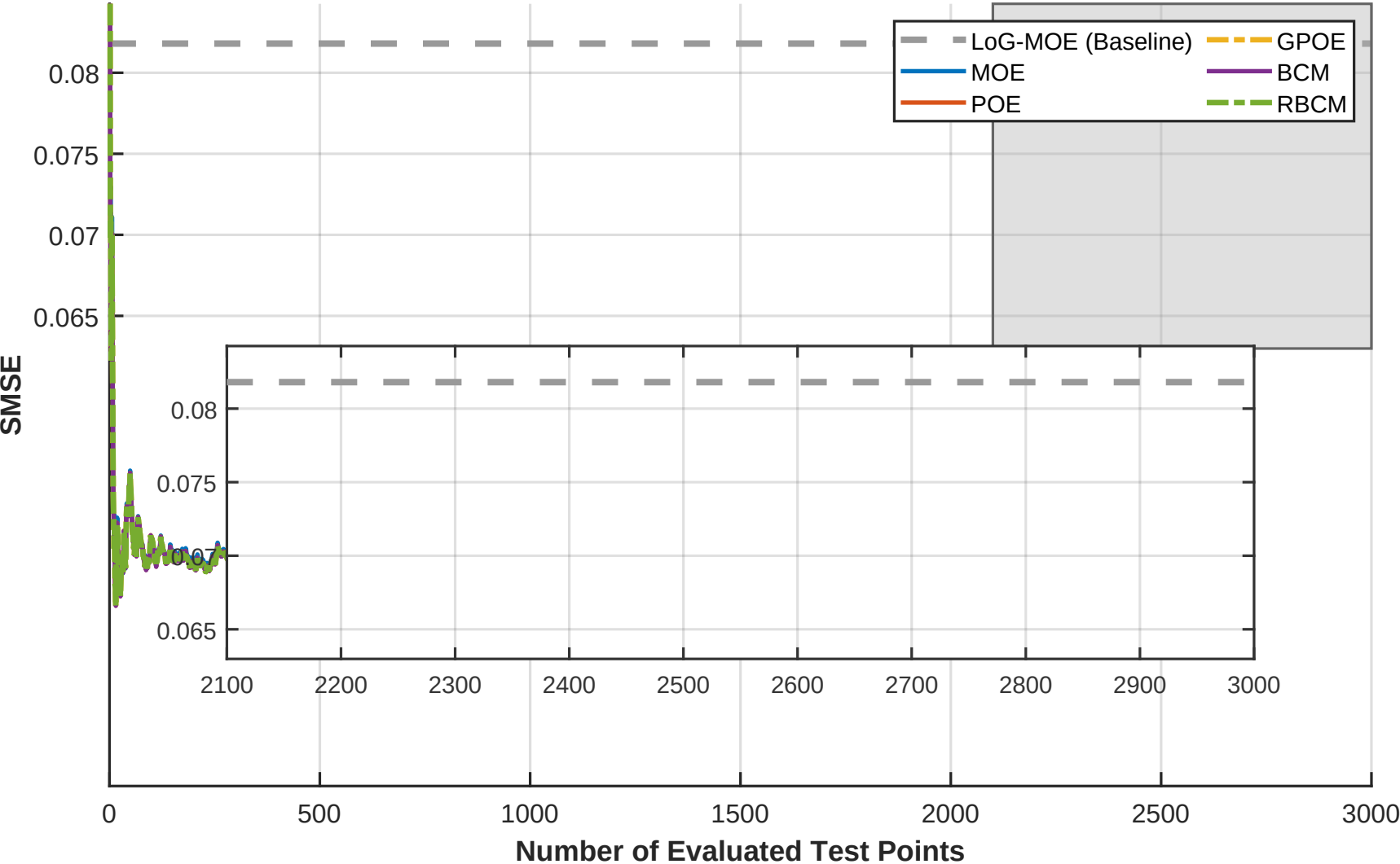
PUMADYN32NM - Fig4 TP DAC - SMSE (5 MC Avg)
