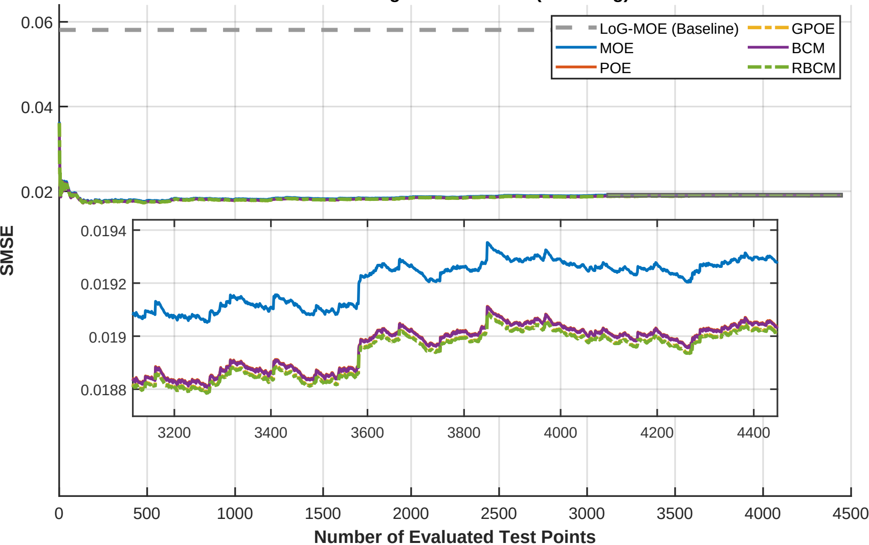
SARCOS - Fig1 IP AC - SMSE (5 MC Avg)
