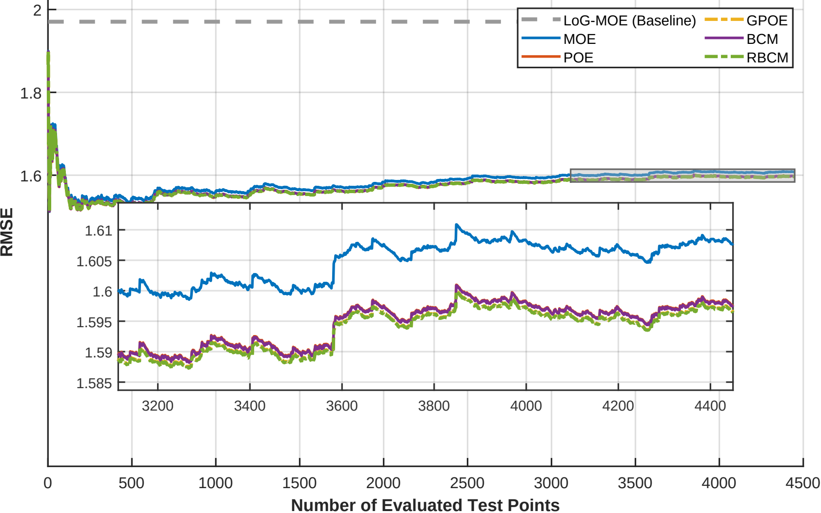
SARCOS - Fig2 IP DAC - RMSE (5 MC Avg)
