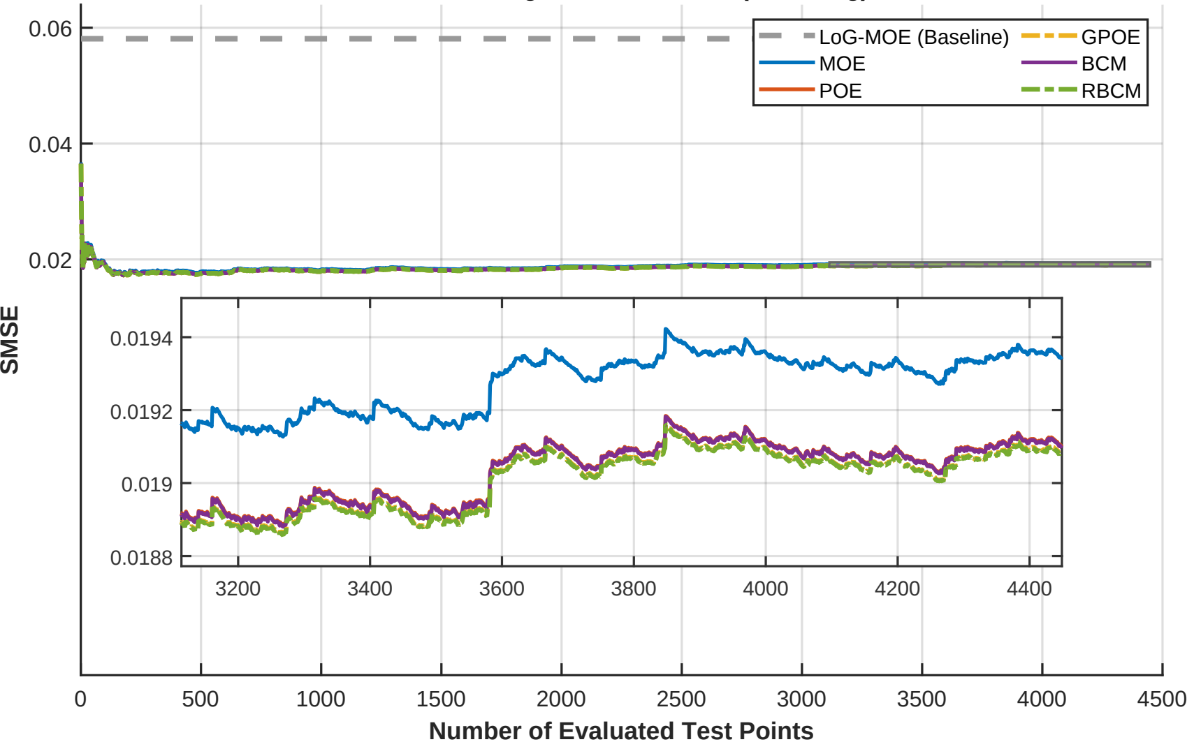
SARCOS - Fig2 IP DAC - SMSE (5 MC Avg)
