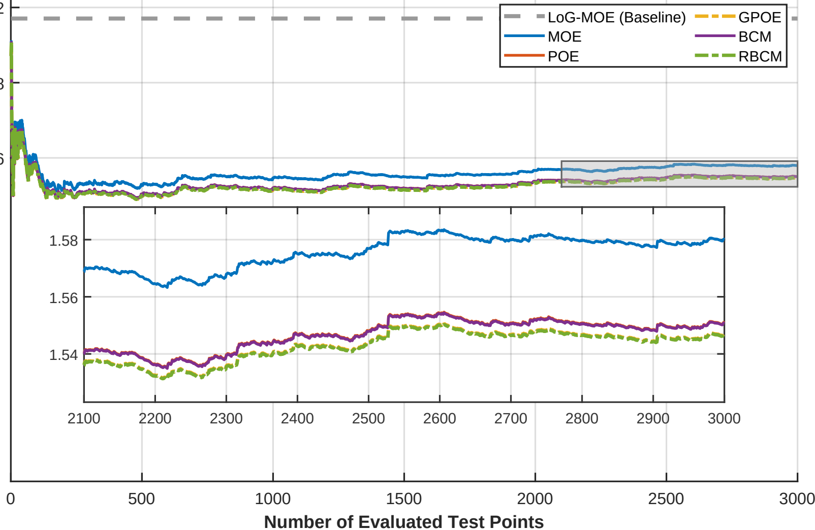
SARCOS - Fig3 TP AC - RMSE (5 MC Avg)
