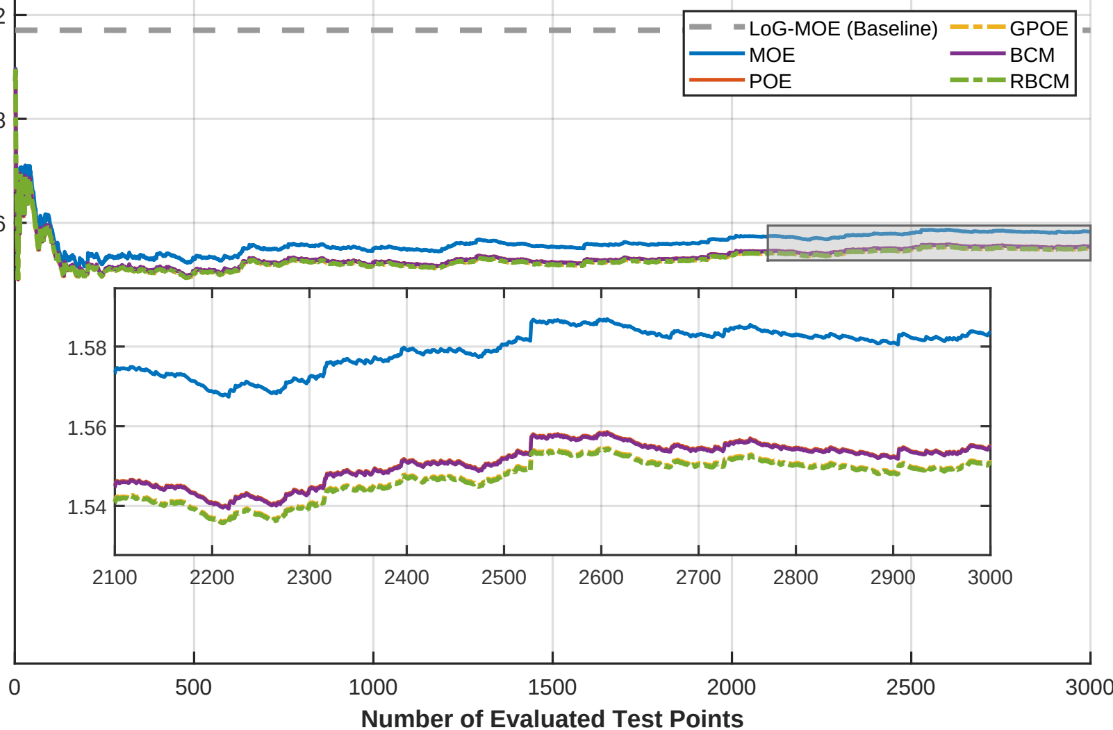
SARCOS - Fig4 TP DAC - RMSE (5 MC Avg)
