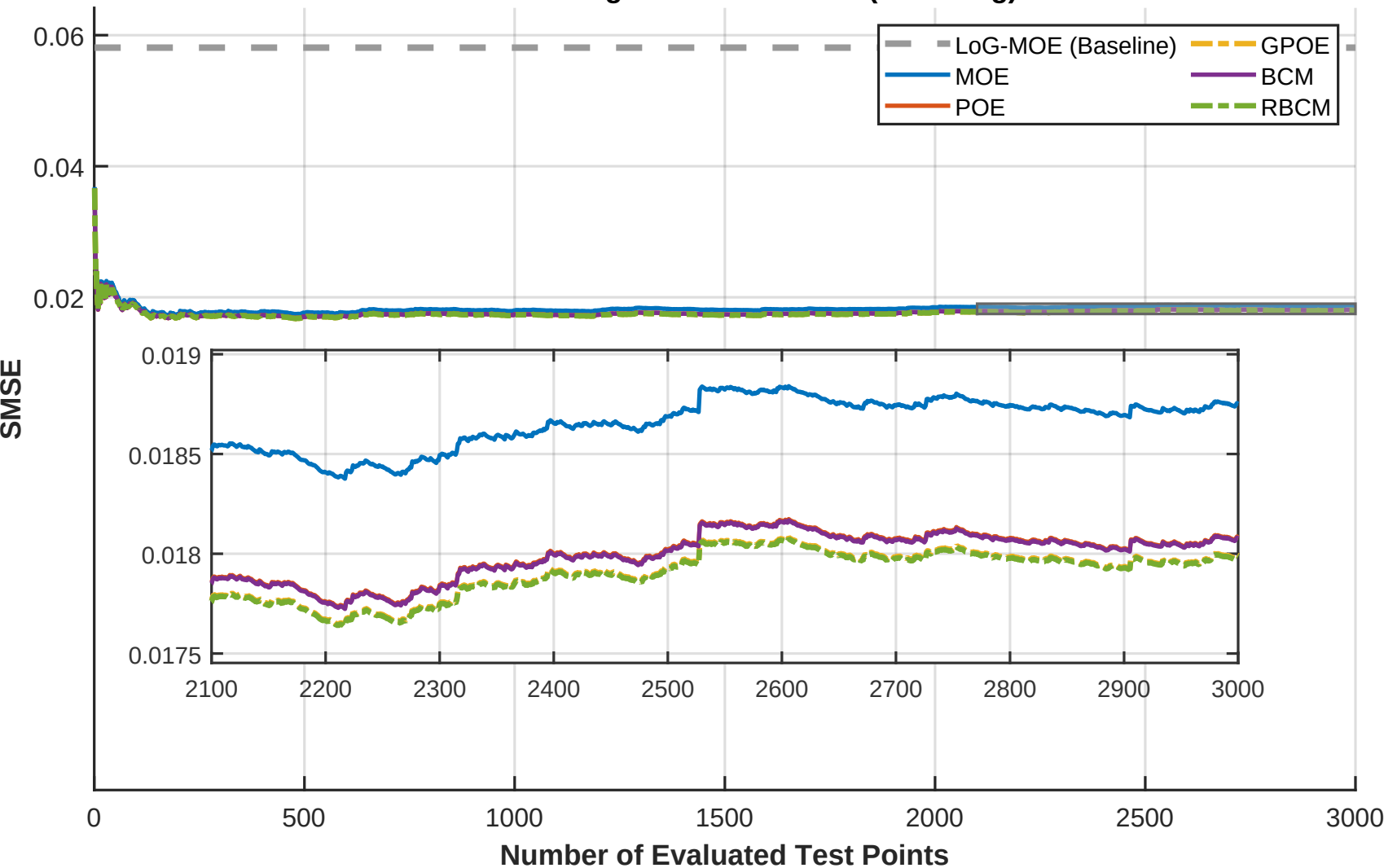
SARCOS - Fig4 TP DAC - SMSE (5 MC Avg)
