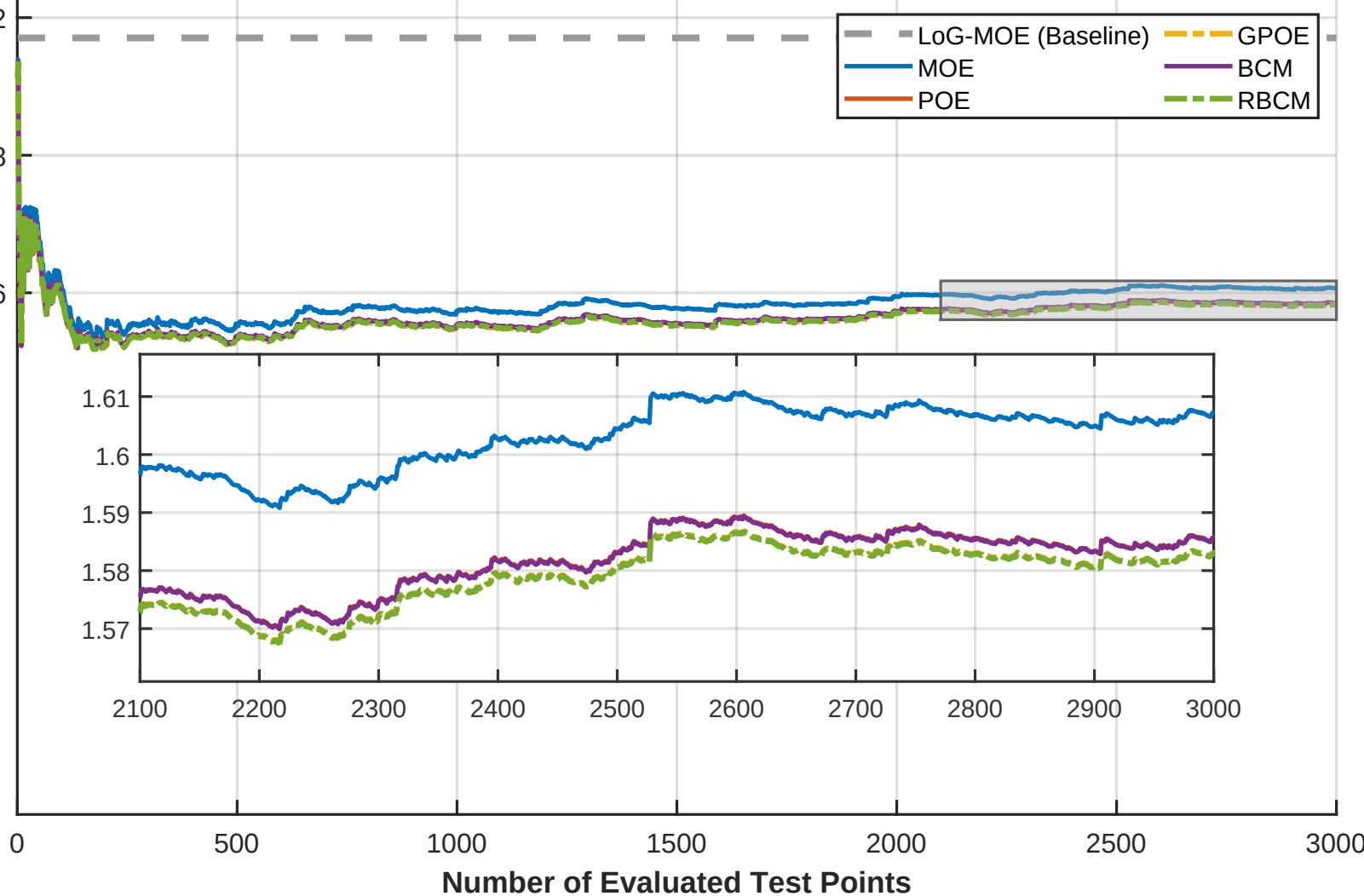
SARCOS - Fig5 Neighbor - RMSE (5 MC Avg)
