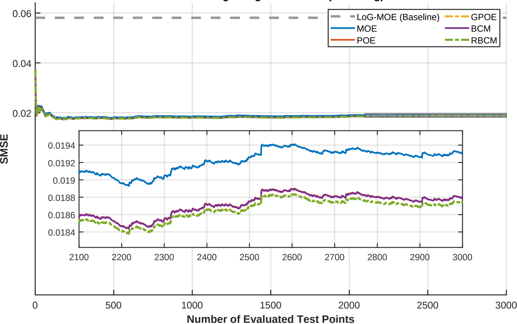
SARCOS - Fig5 Neighbor - SMSE (5 MC Avg)
