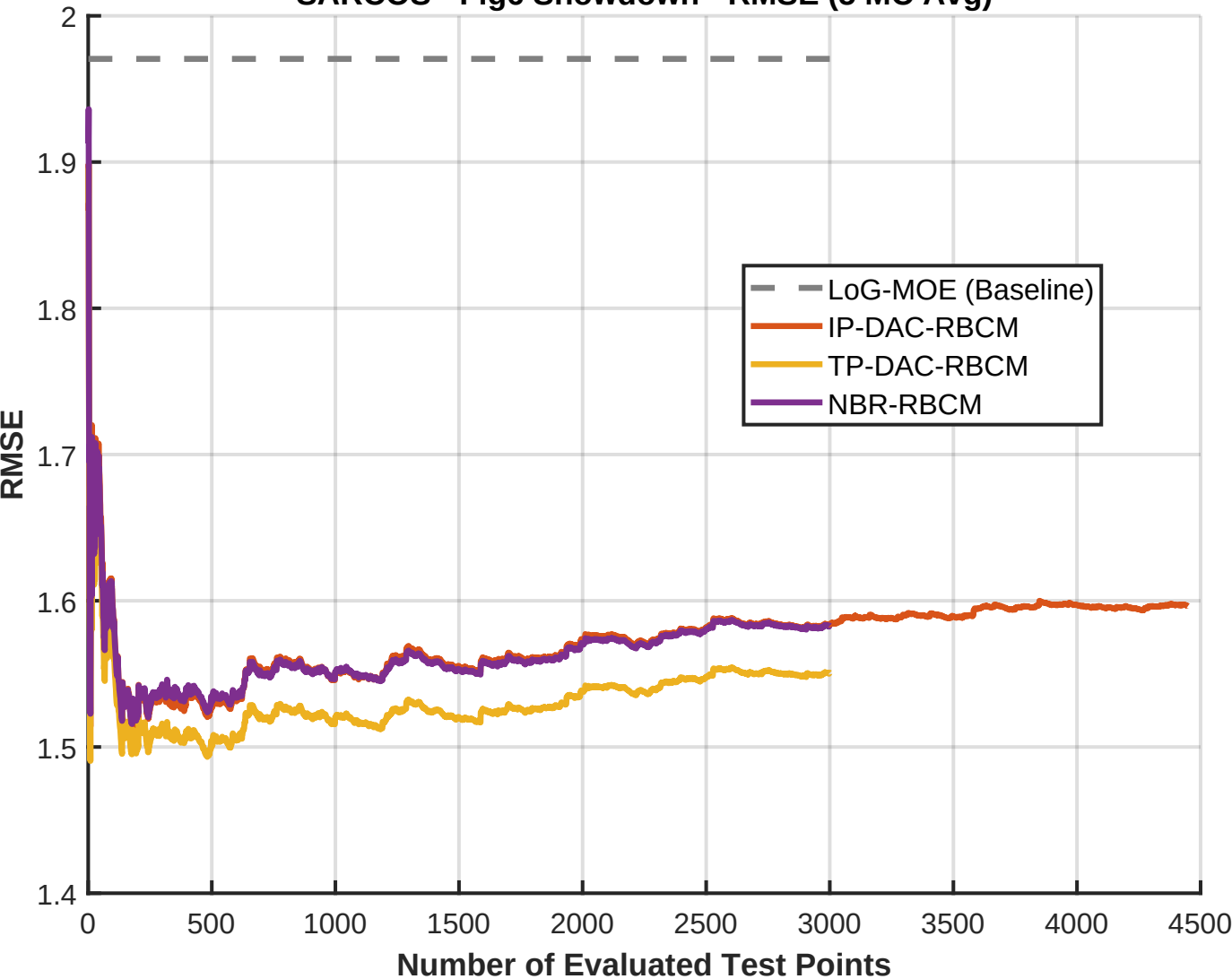
SARCOS - Fig6 Showdown - RMSE (5 MC Avg)
