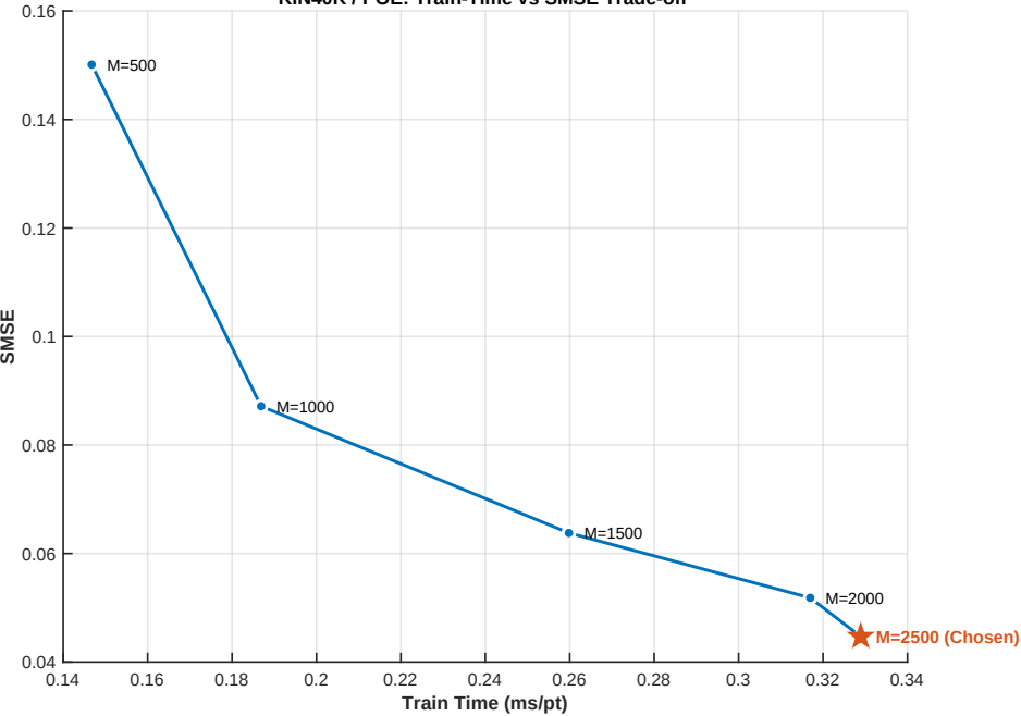
KIN40K / POE: Train-Time vs SMSE Trade-off
