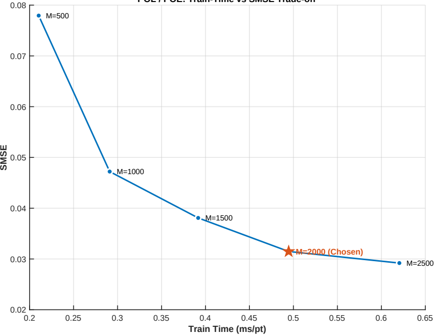
POL / POE: Train-Time vs SMSE Trade-off
