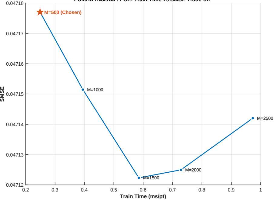
PUMADYN32NM / POE: Train-Time vs SMSE Trade-off
