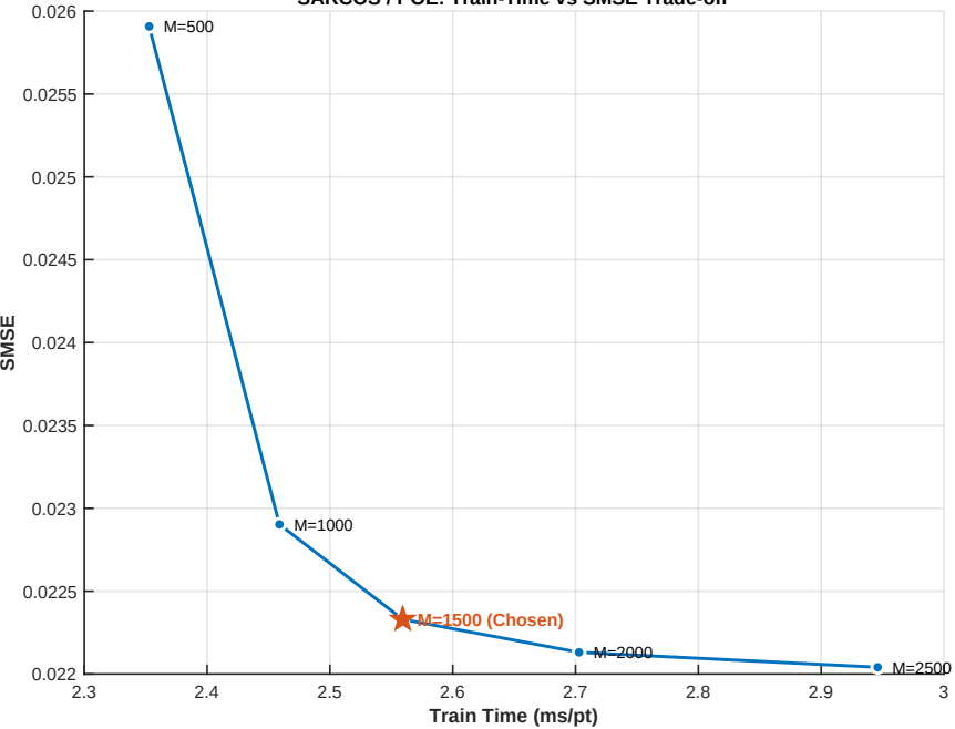
SARCOS / POE: Train-Time vs SMSE Trade-off
