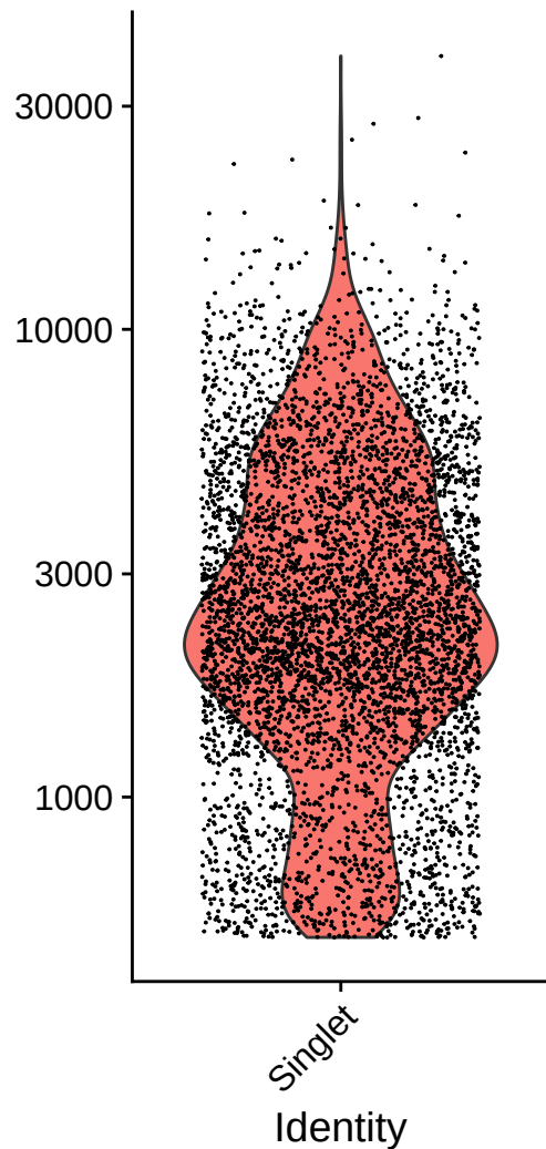
nCount_RNA
