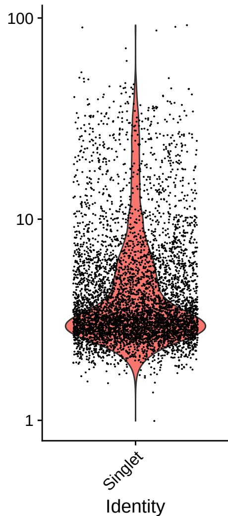
percent.mt
