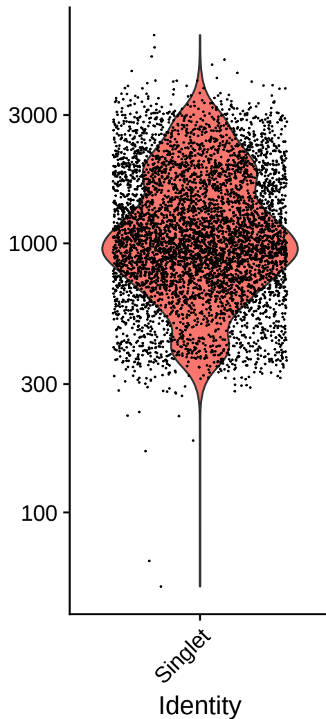
nFeature_RNA
