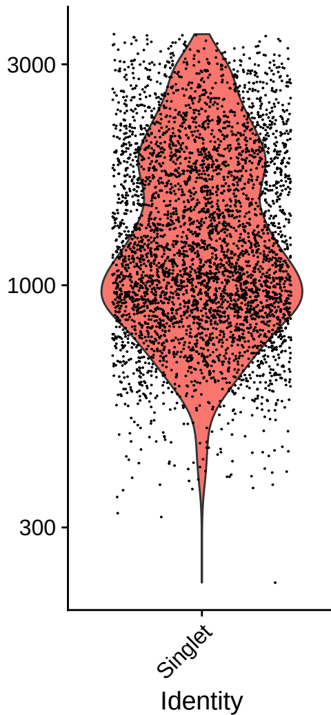
nFeature_RNA
