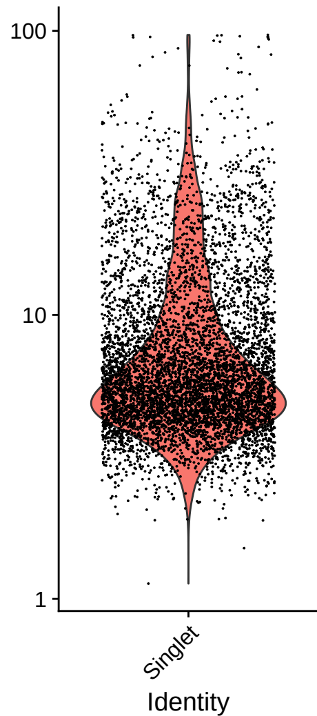
percent.mt
