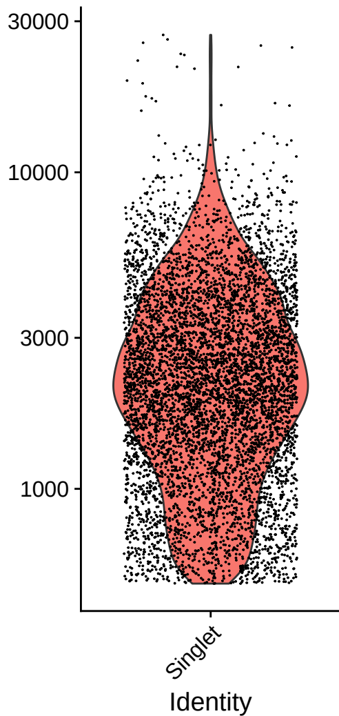
nCount_RNA
