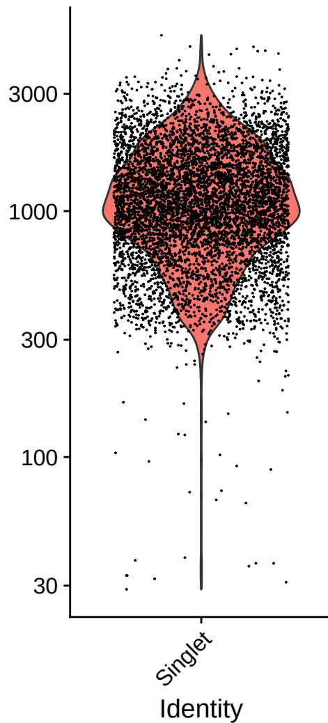
nFeature_RNA
