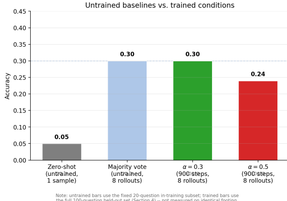
Figure 2: Untrained zero-shot and untrained majority-vote accuracy (gray / light blue) versus final accuracy after 900 steps of training at \alpha=0.3 and \alpha=0.5 (green / red). The untrained bars use the fixed 20-question in-training subset; the trained bars use the full 100-question held-out set (Section 4), so the comparison is directional rather than exact.
