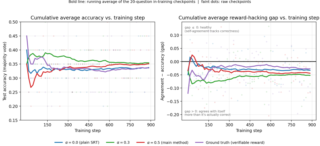
Figure 1: Cumulative (running) average of test accuracy (left) and agreement-accuracy gap (right) vs. training step, for all four conditions, including the ground-truth condition. Each bold line is the running mean of that condition’s 20-question in-training checkpoints (every 15 steps, fixed seed) from step 0 up to the current step; faint dots are the raw, unsmoothed checkpoints, shown to make the per-checkpoint sampling noise visible rather than hiding it. Gap is agreement minus accuracy (Section 2): positive means the model agrees with itself more than it is actually correct, the reward-hacking signature. The low-noise, 100-question final evaluation for each condition is reported separately in Table 2 rather than overlaid here.
