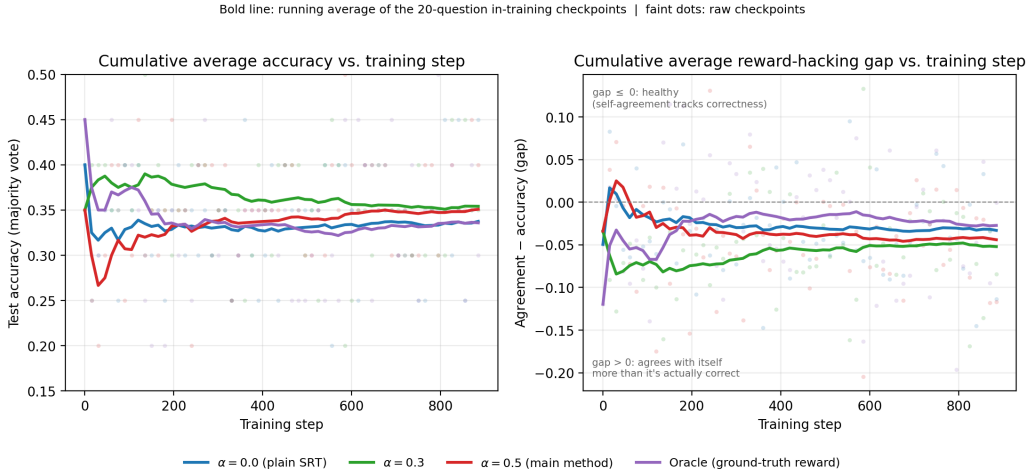
Figure 1: Cumulative (running) average of test accuracy (left) and agreement-accuracy gap (right) vs. training step, for all four conditions, including the oracle. Each bold line is the running mean of that condition’s 20-question in-training checkpoints (every 15 steps, fixed seed) from step 0 up to the current step; faint dots are the raw, unsmoothed checkpoints, shown to make the per-checkpoint sampling noise visible rather than hiding it. Gap is agreement minus accuracy (Section 2): positive means the model agrees with itself more than it is actually correct, the reward-hacking signature. The low-noise, 100-question final evaluation for each condition is reported separately in Table 2 rather than overlaid here.
