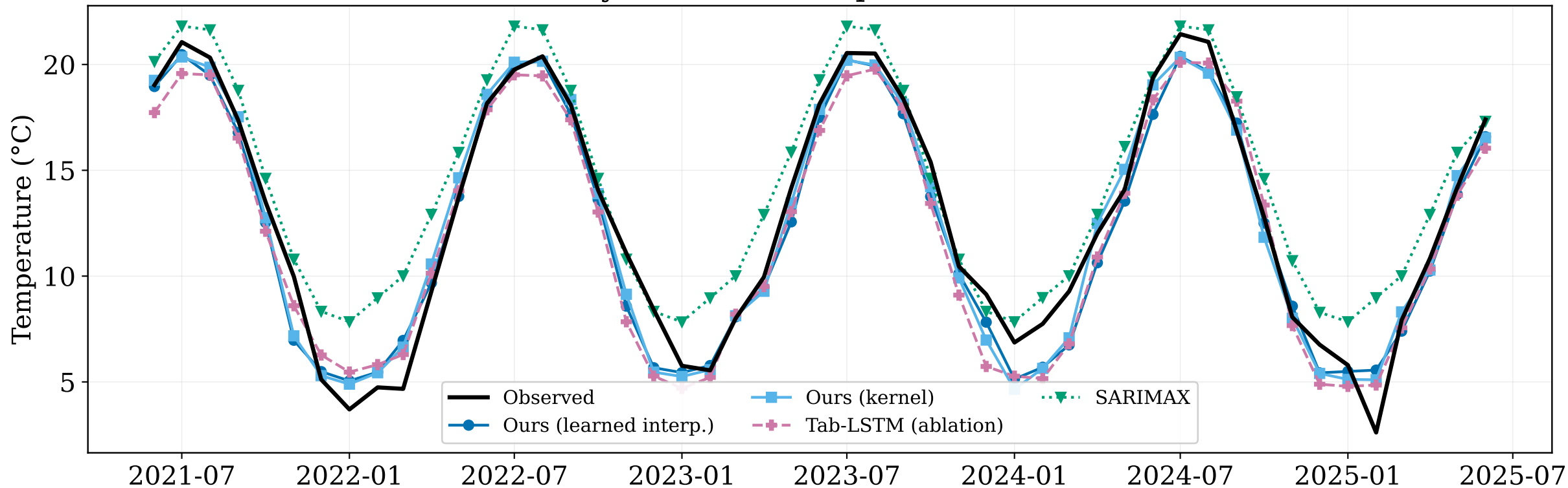
Monthly Minimum Temperature — Center
