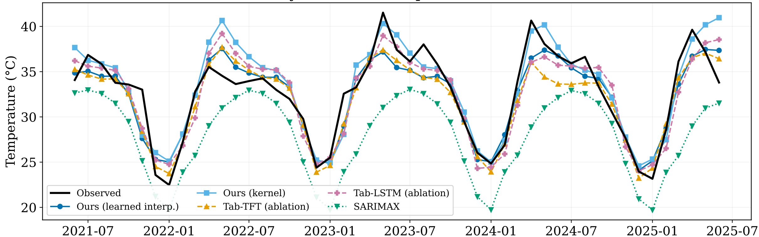
Monthly Maximum Temperature — Center
