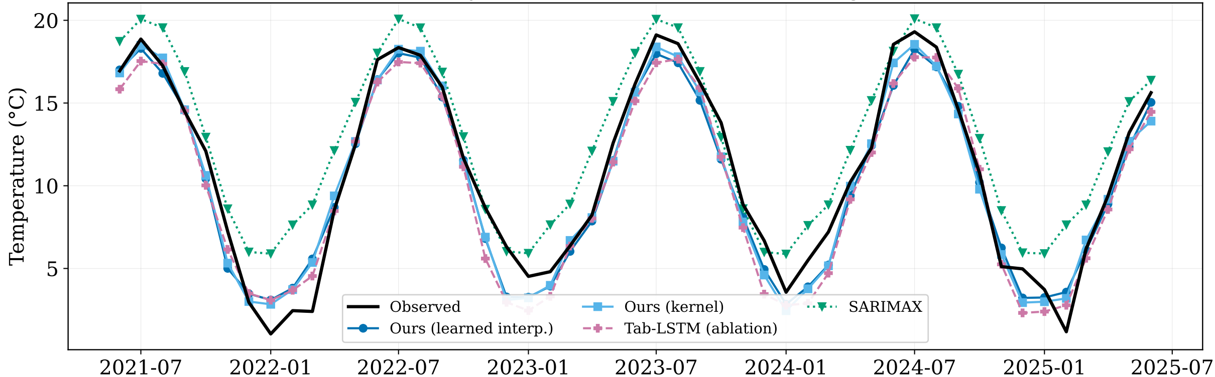
Monthly Minimum Temperature — Negev
