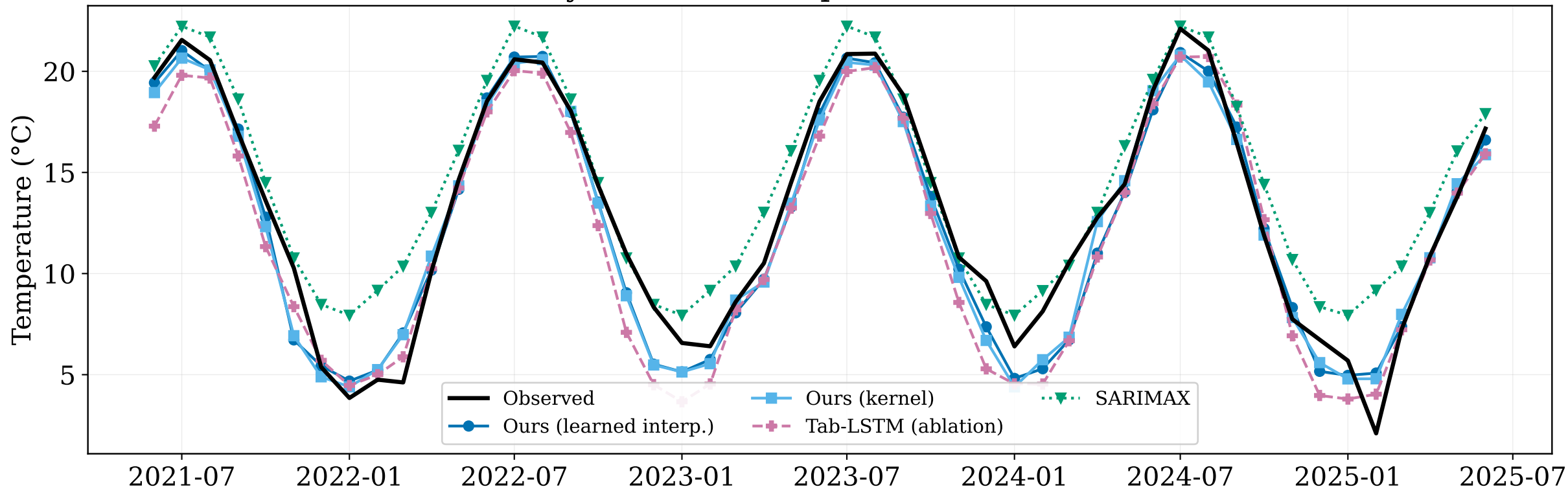
Monthly Minimum Temperature — North-West
