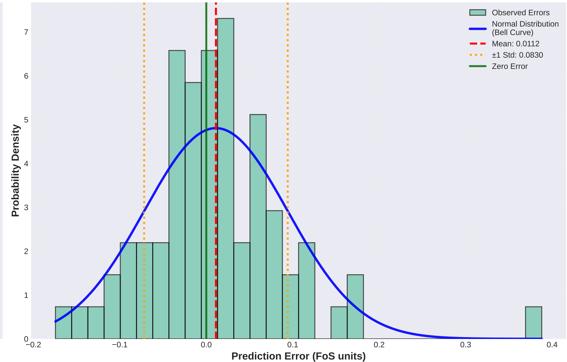
XGBoost - Error Distribution (n=73)
