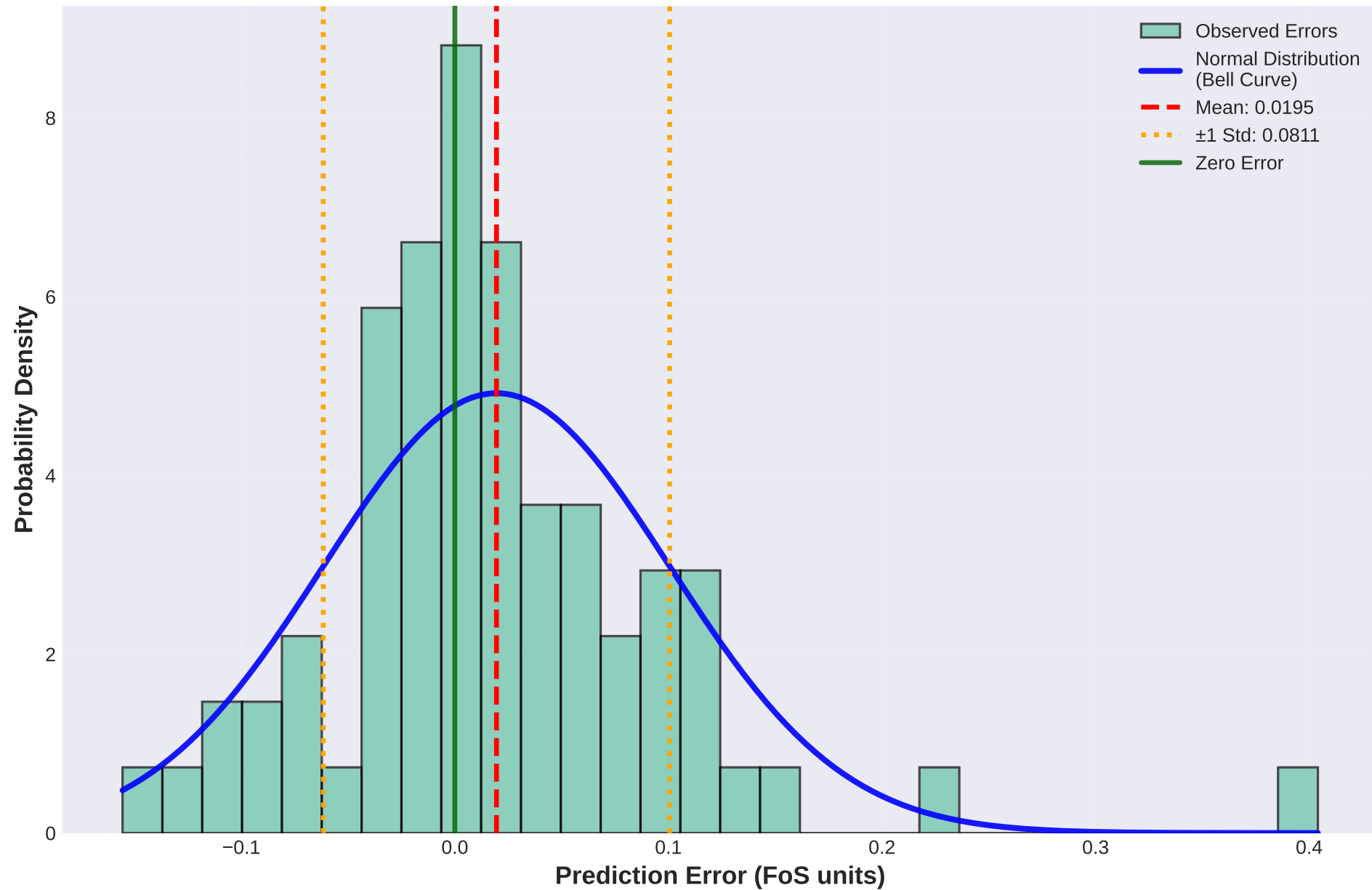
Gradient Boosting - Error Distribution (n=73)
