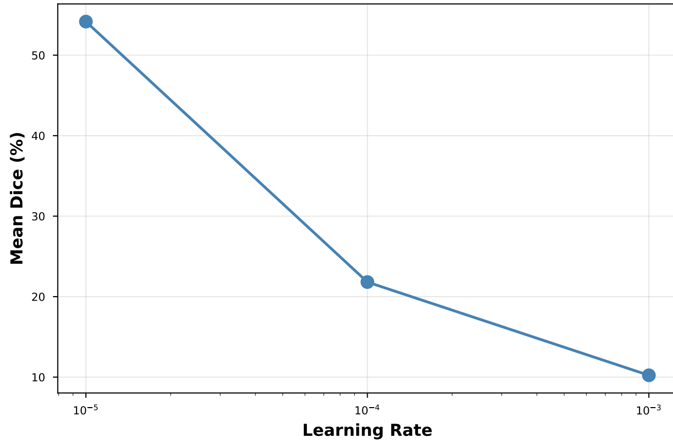
Learning Rate Sensitivity
