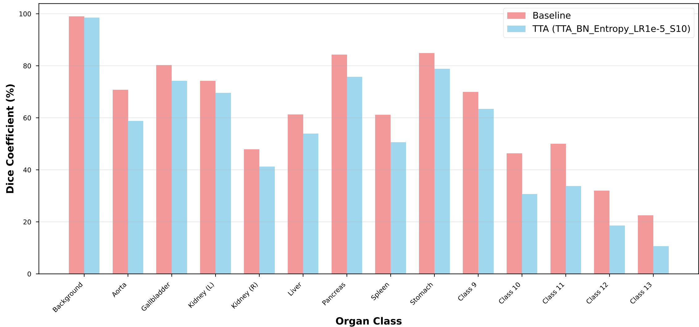
Per-Class Performance: Baseline vs TTA
