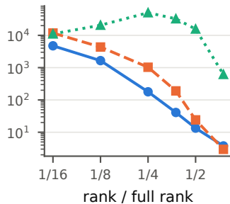
SmolLM2-1.7B
