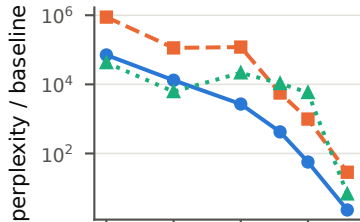
SmolLM2-135M
