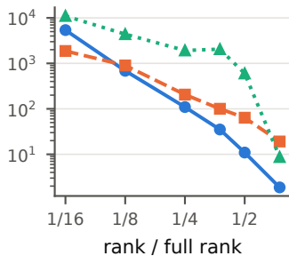
Qwen2.5-1.5B
