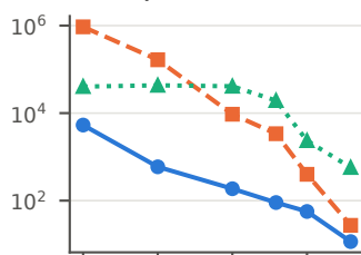
Qwen2.5-0.5B
