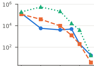
SmolLM2-360M
