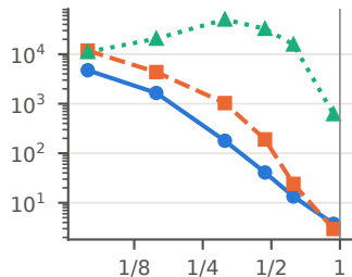
SmolLM2-1.7B
