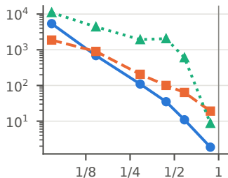
Qwen2.5-1.5B
