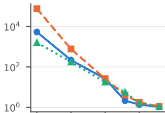
SmolLM2-360M
