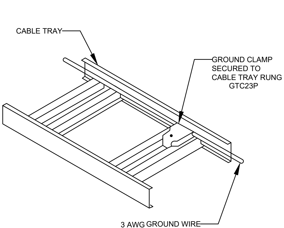
CABLE TRAY GROUND CLAMP
