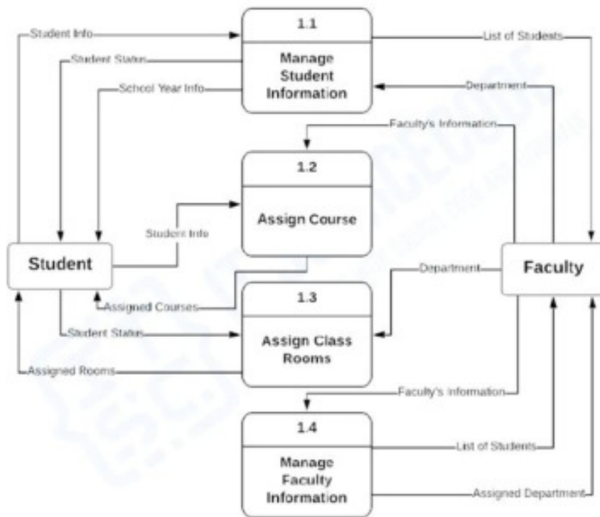
University Management System DFD Level 1
