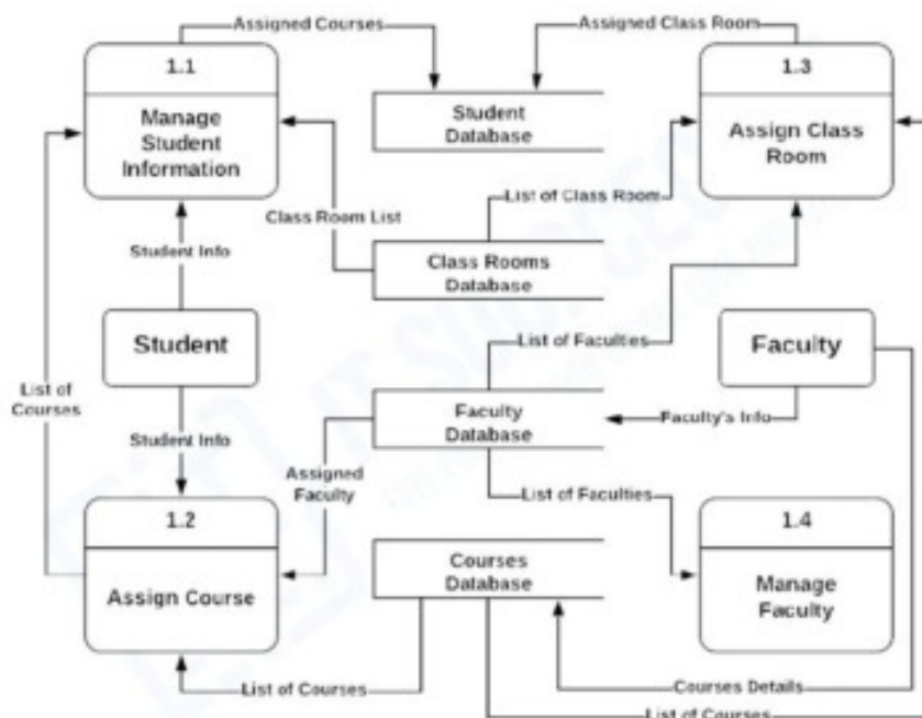
University Management System DFD Level 2
