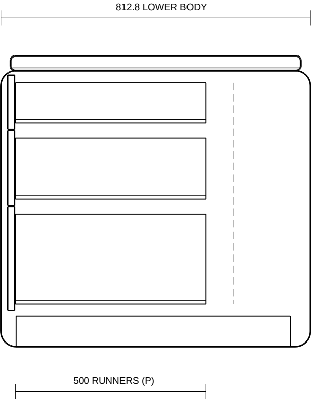
A-A / PEDESTAL SECTION
