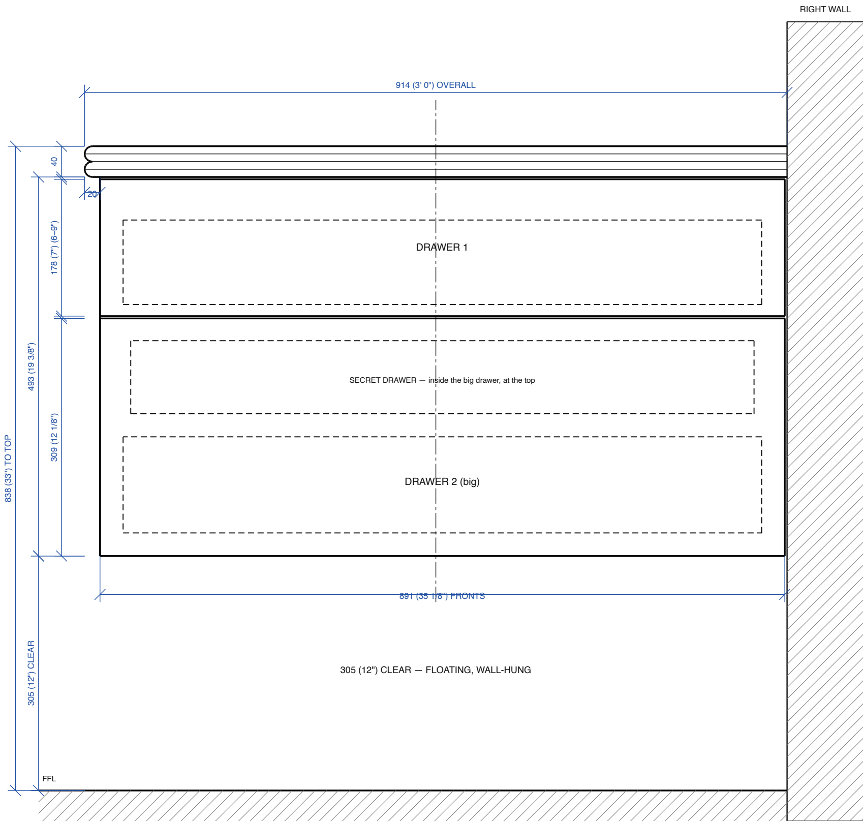
FRONT ELEVATION
