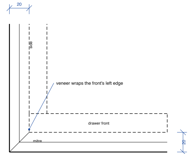
DETAIL 2 — FRONT-LEFT CORNER, PLAN
