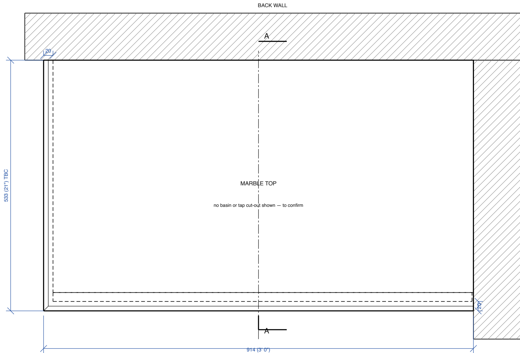
PLAN SCALE 1:5 at A3
