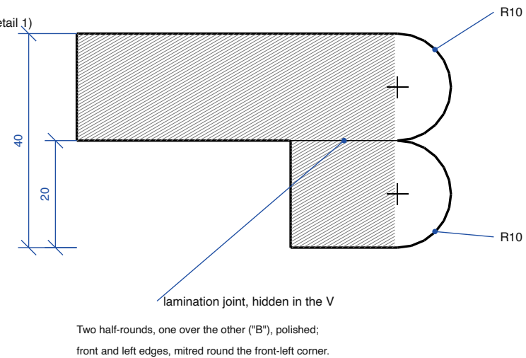
DETAIL 1 — STONE EDGE "B"
