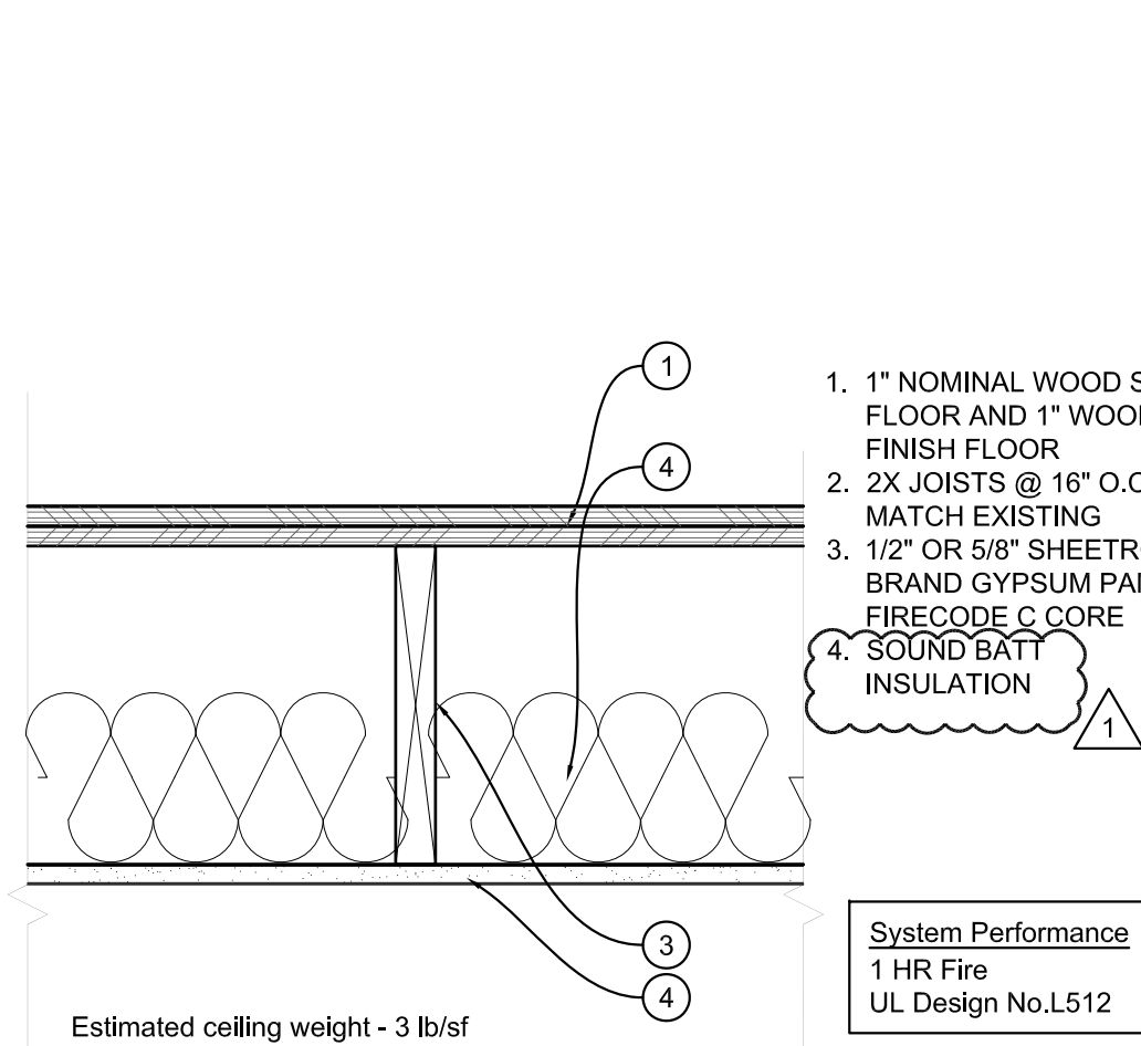
D3 DECK TYPE 1 HR RATED
