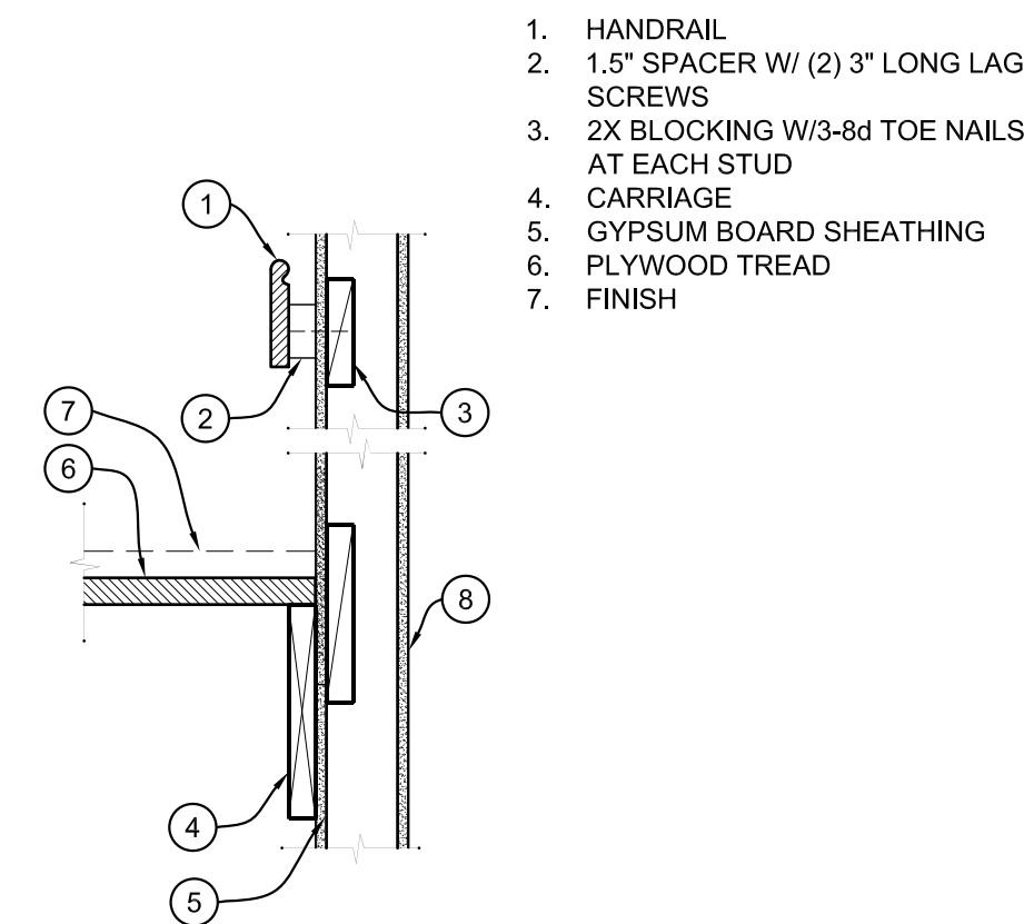
4 STAIR DETAIL
