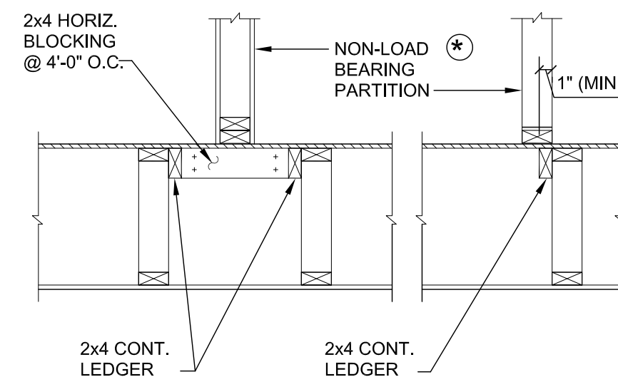
2 TYP. NON-LOAD BEARING PARTITION PARALLEL TO TRUSSES OR JOISTS
