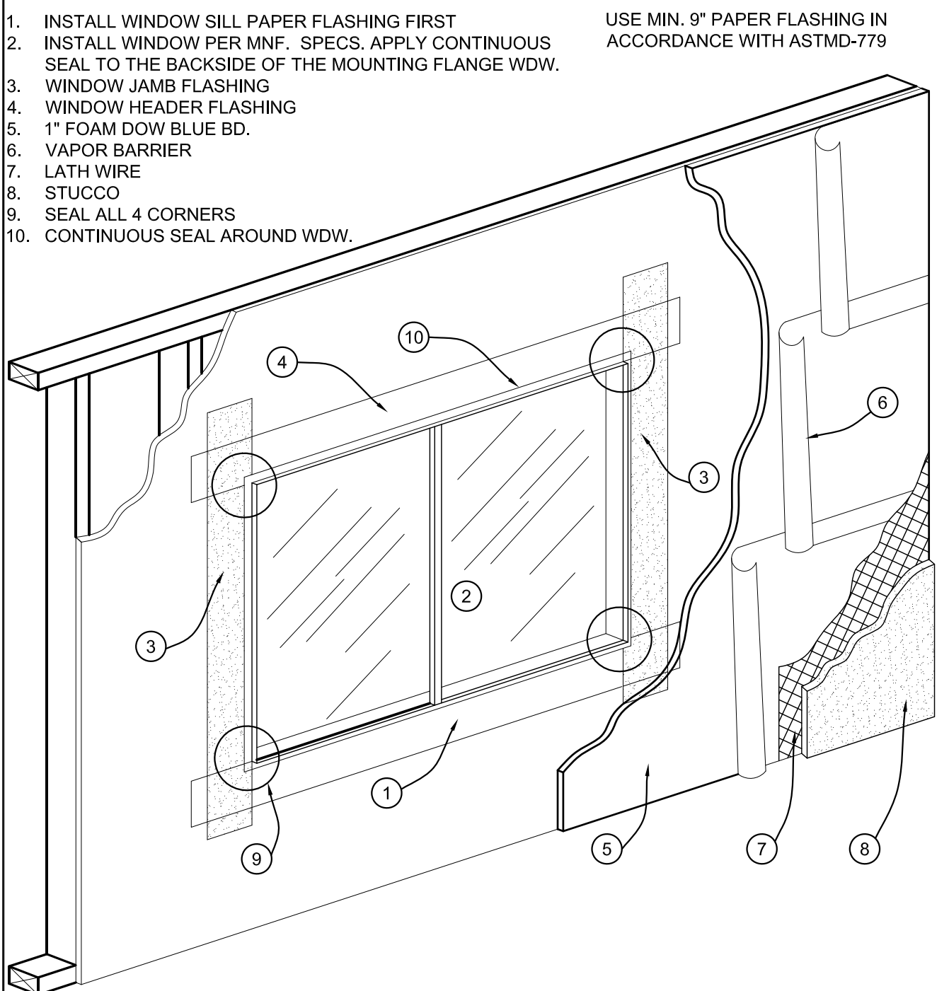
9 WINDOW FLASHING DETAIL
