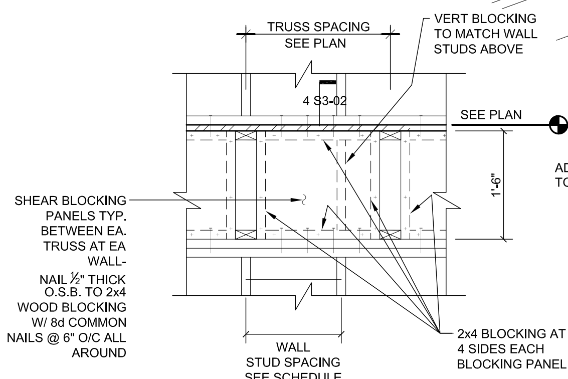
8 TYP. SHEAR BLOCKING PANELS
