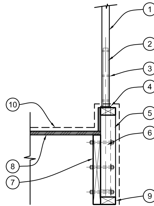
A SECTION A
