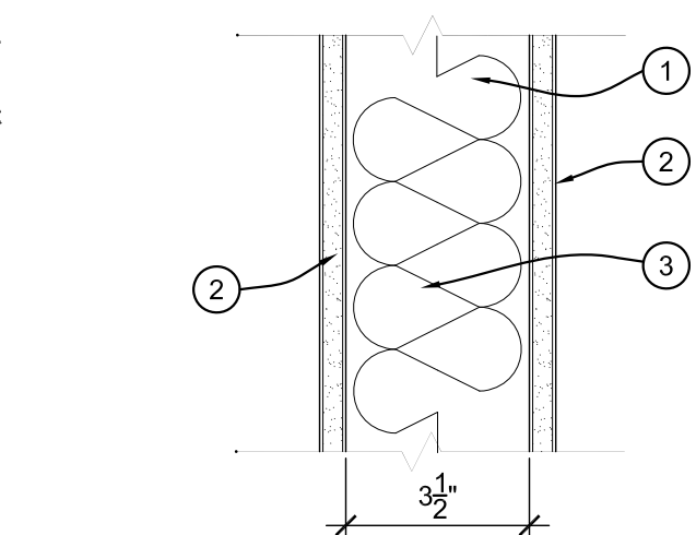
P1 PARTITION TYPE "P1"
