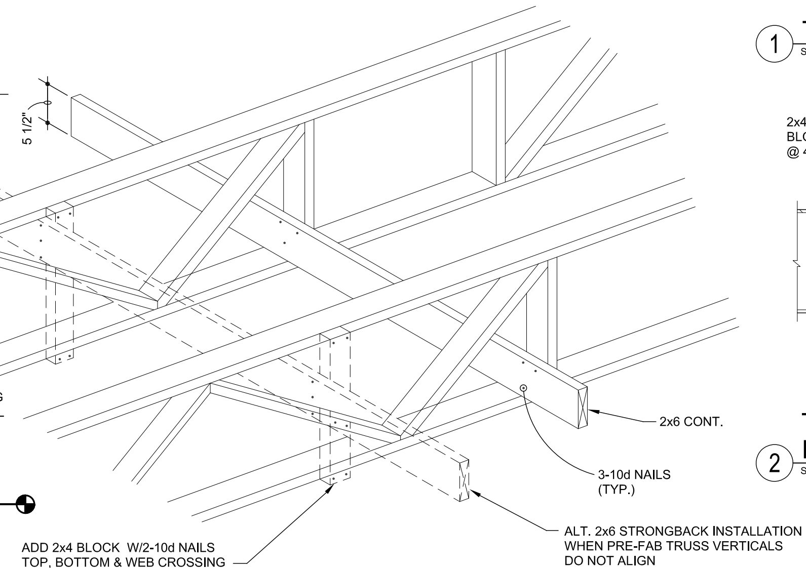
5 APPLICATION OF STRONGBACK (10'-0" O.C. MAX.)
