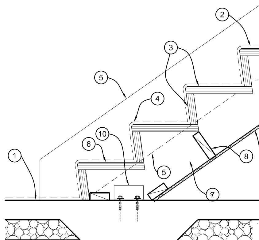
2 STAIR STRINGER TO CONC. SLAB
