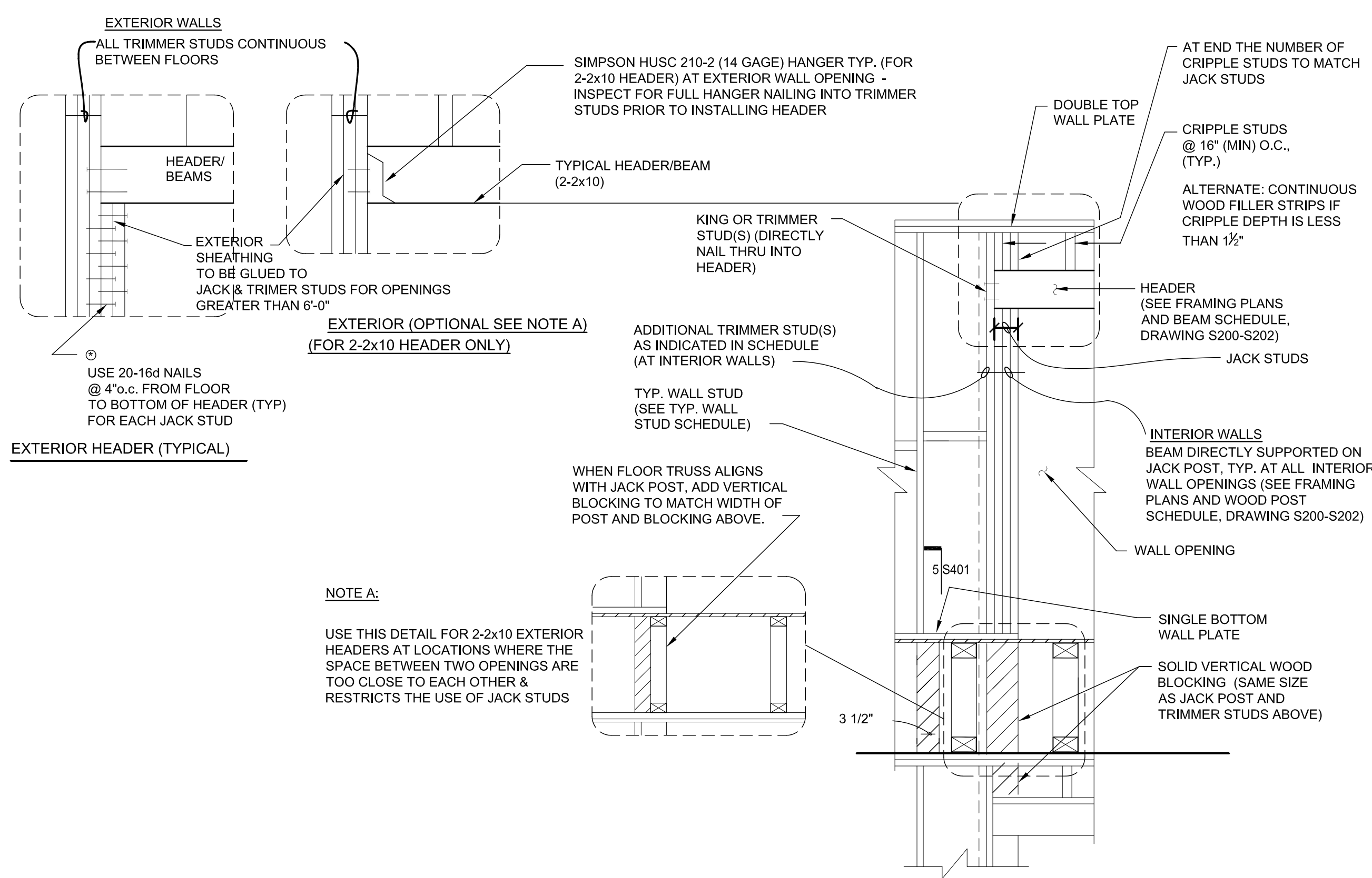
1 TYP. JACKPOST/BLOCKING
