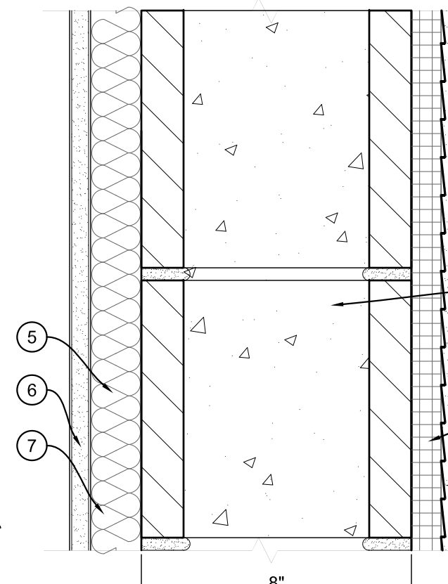
W3 WALL-TYPE W3
