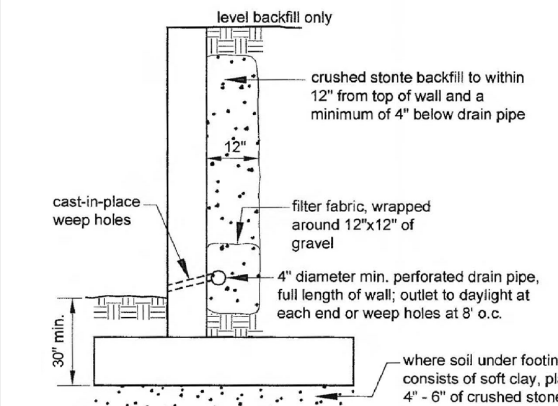
11 MASONRY, CONCRETE WALL BACKFILL AND DRAINAGE SCALE: N.T.S.
