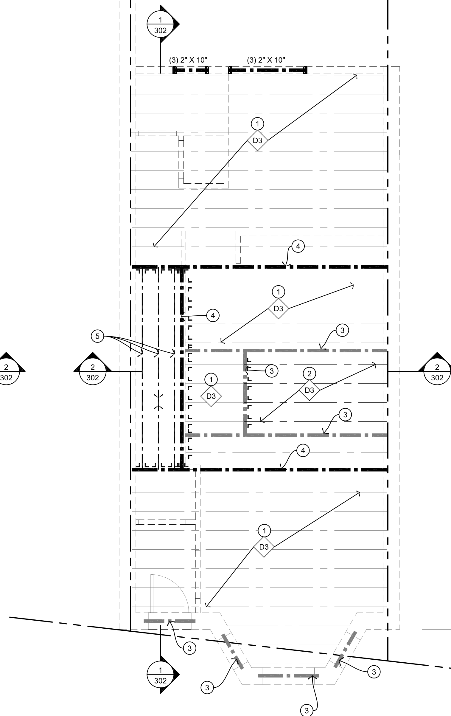
2ND FLOOR FRAMING PLAN
