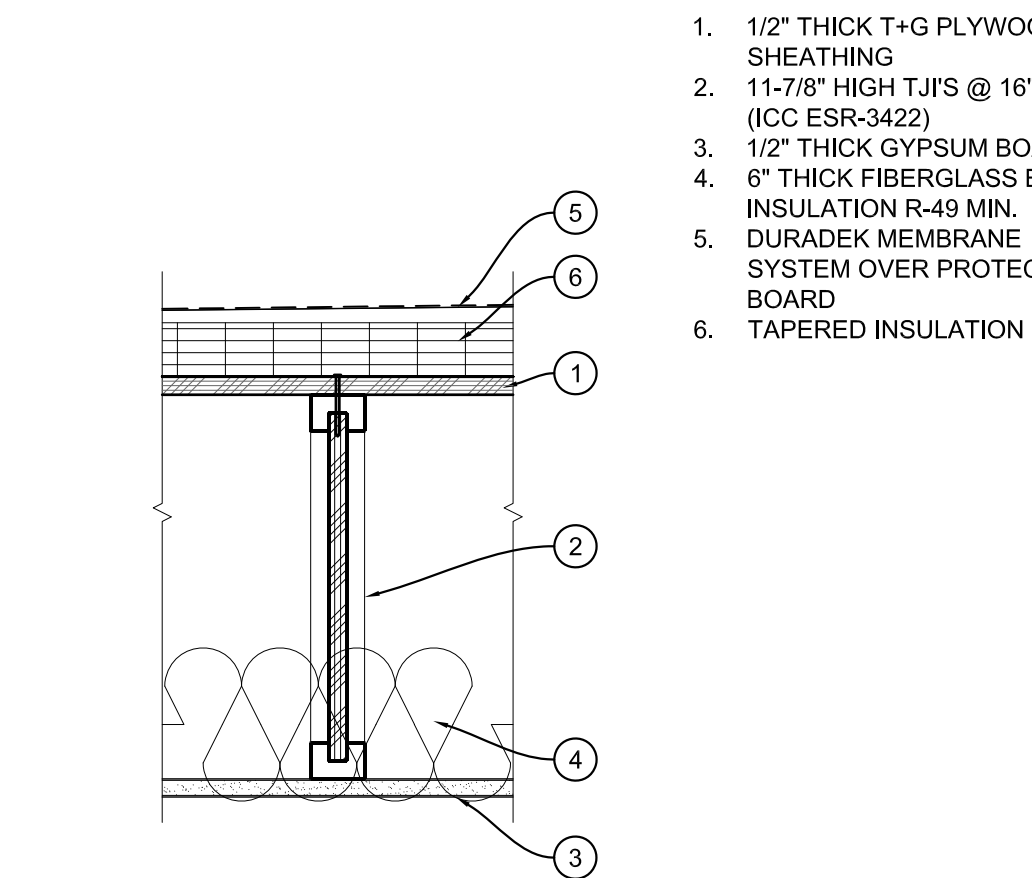
D3 DECK TYPE 1 HR RATED
