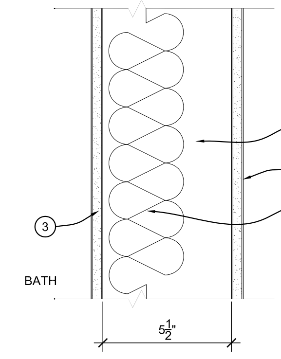
P2 PARTITION TYPE "P2"
