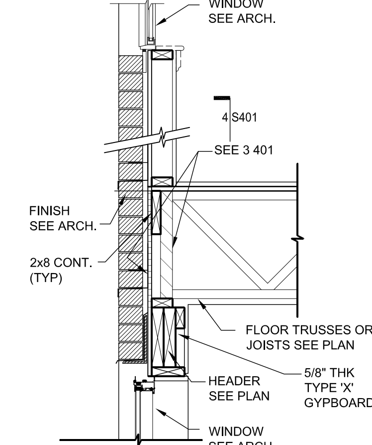
9 WINDOW SILL & HEADER DETAIL
