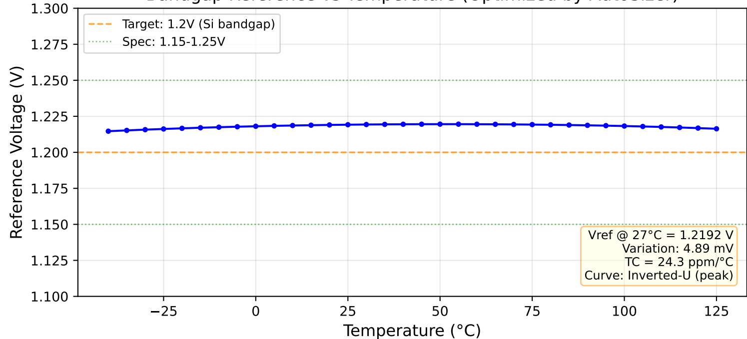
Bandgap Reference vs Temperature (Optimized by AutoSizer)
