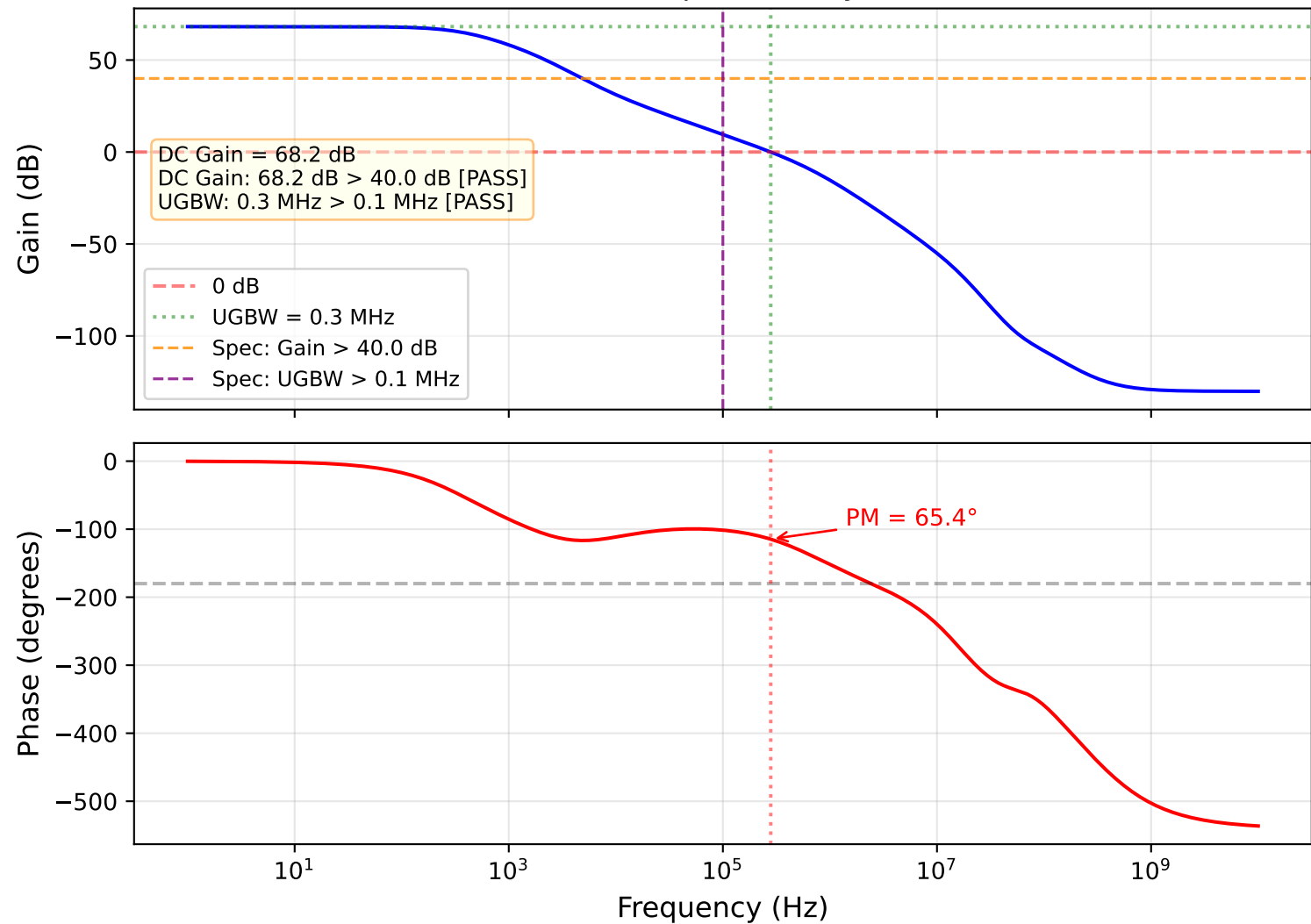
iac - Bode Plot (Optimized by AutoSizer)
