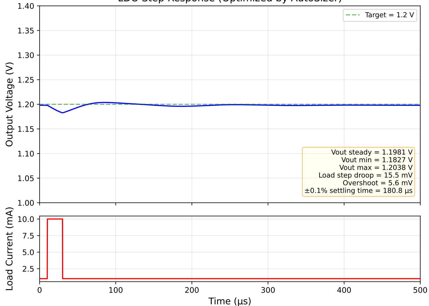
LDO Step Response (Optimized by AutoSizer)
