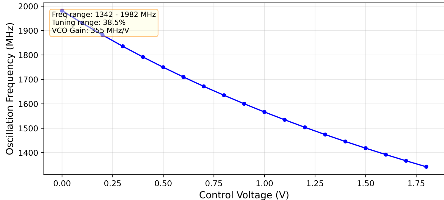
VCO Tuning Curve (Optimized by AutoSizer)
