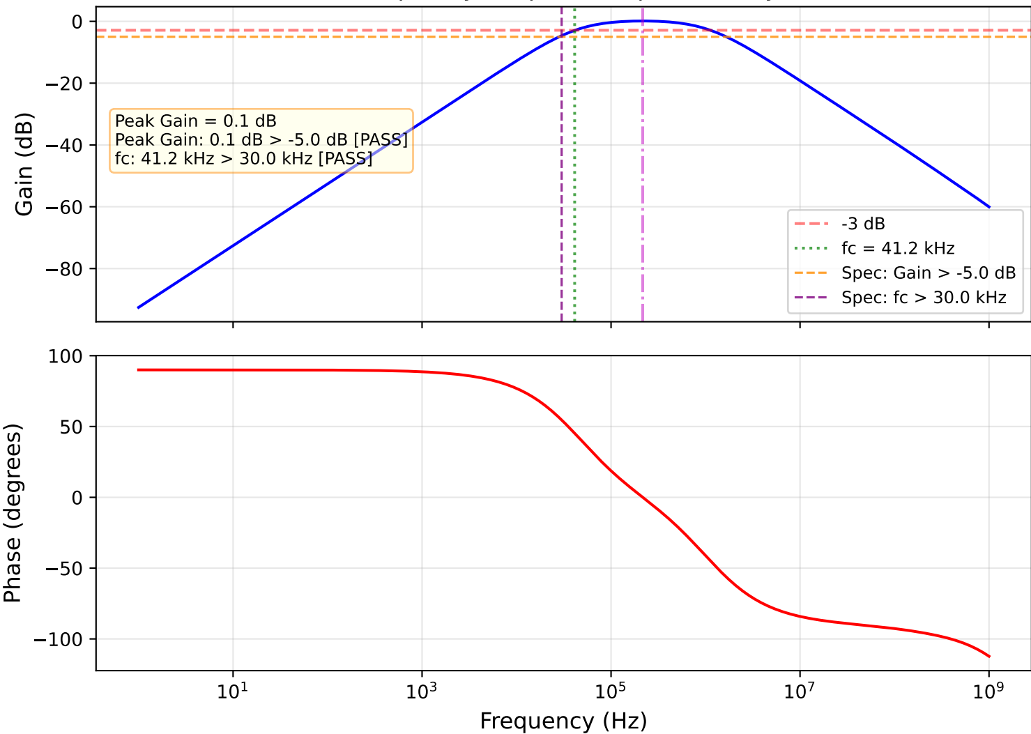
BPF Filter - Frequency Response (Optimized by AutoSizer)
