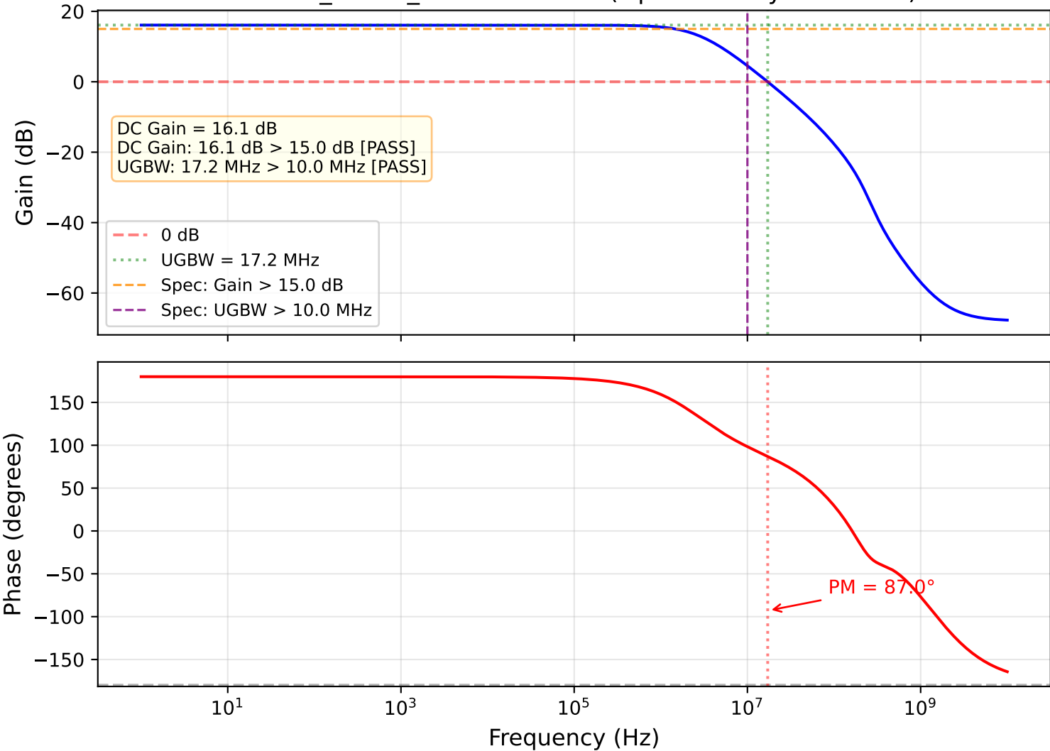
current_mirror_ota - Bode Plot (Optimized by AutoSizer)
