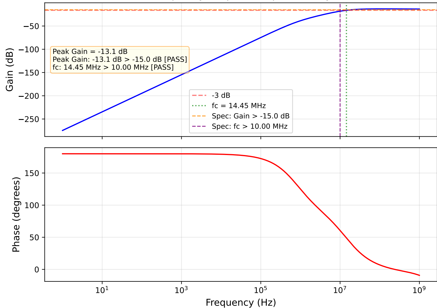
HPF Filter - Frequency Response (Optimized by AutoSizer)
