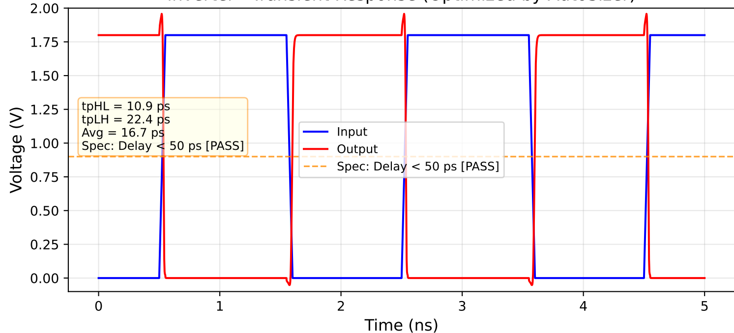
inverter - Transient Response (Optimized by AutoSizer)
