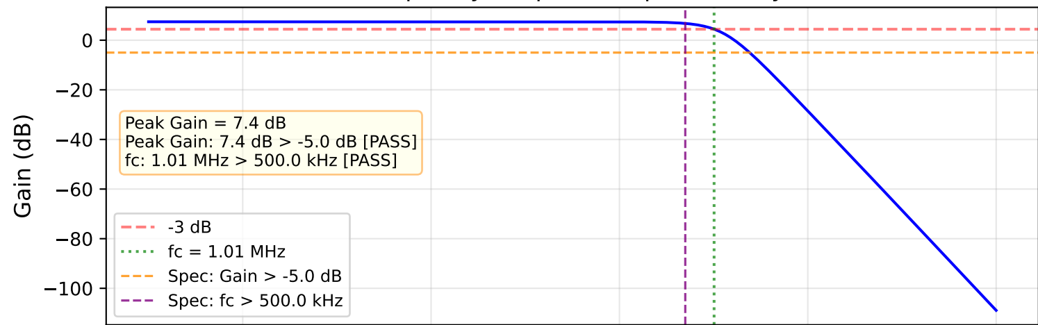
LPF Filter - Frequency Response (Optimized by AutoSizer)
