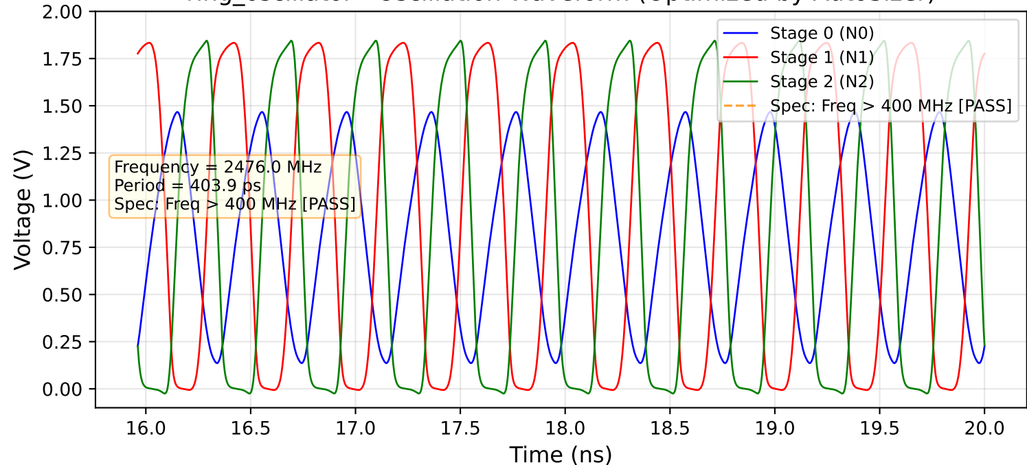
ring_oscillator - Oscillation Waveform (Optimized by AutoSizer)
