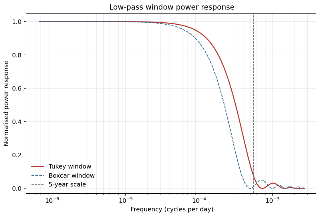
Tukey and boxcar filter response
