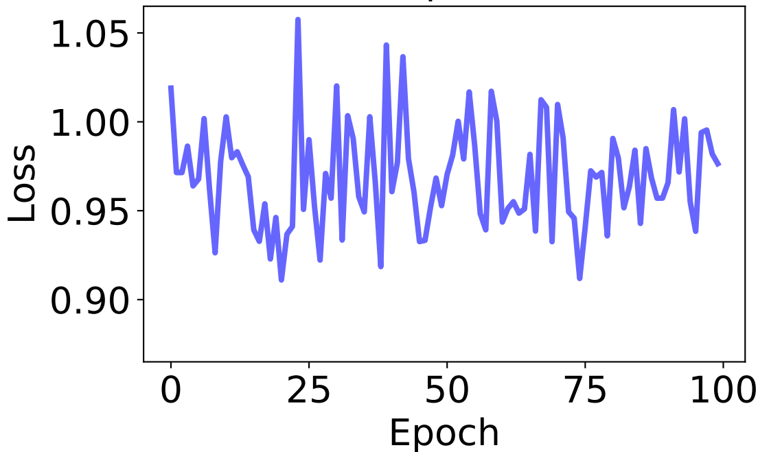
SGD ( \eta = 0.01 )
