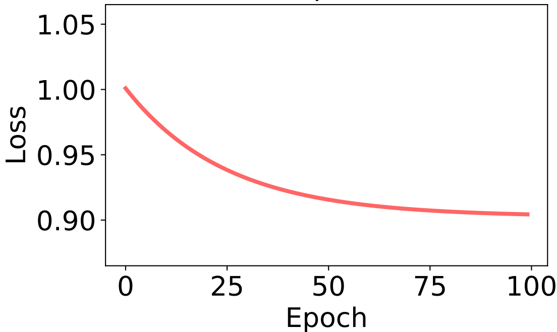
BGD ( \eta = 0.01 )
