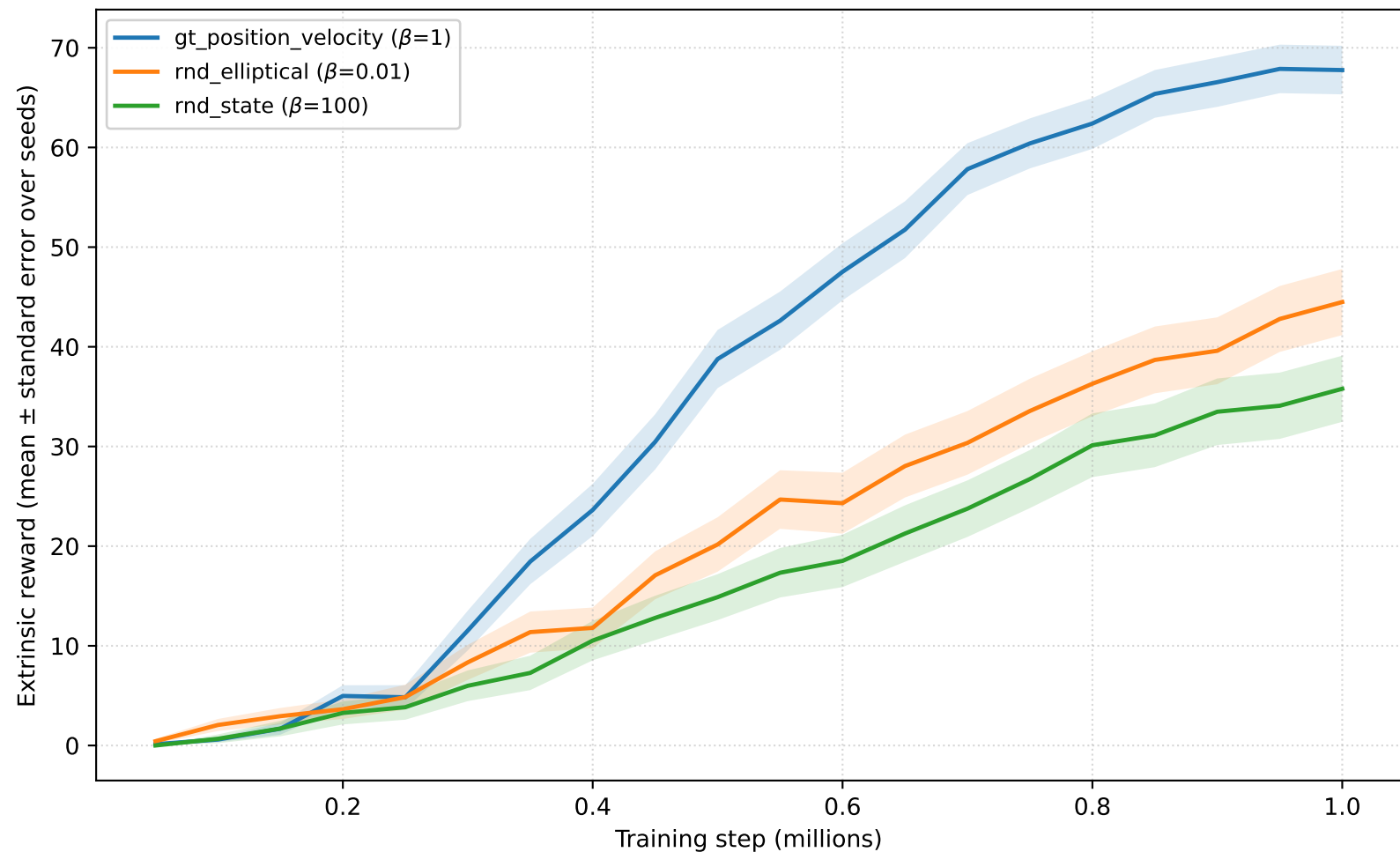
Train run 2: reward over training (eval; each line up to n \geq 30 seeds)
