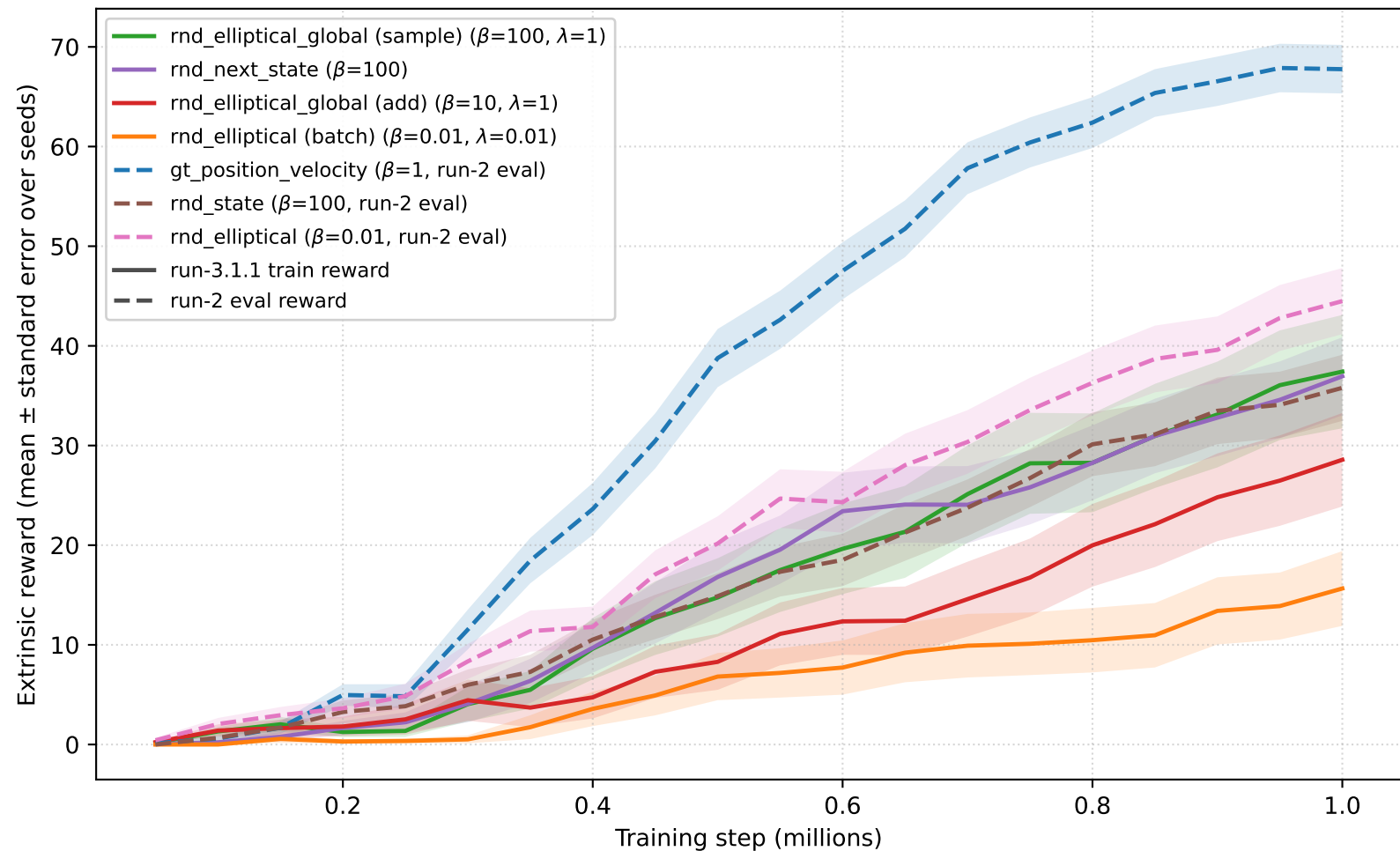
Train run 3.1.1: training-episode reward per method at its best config (each line up to n \geq 30 seeds)
