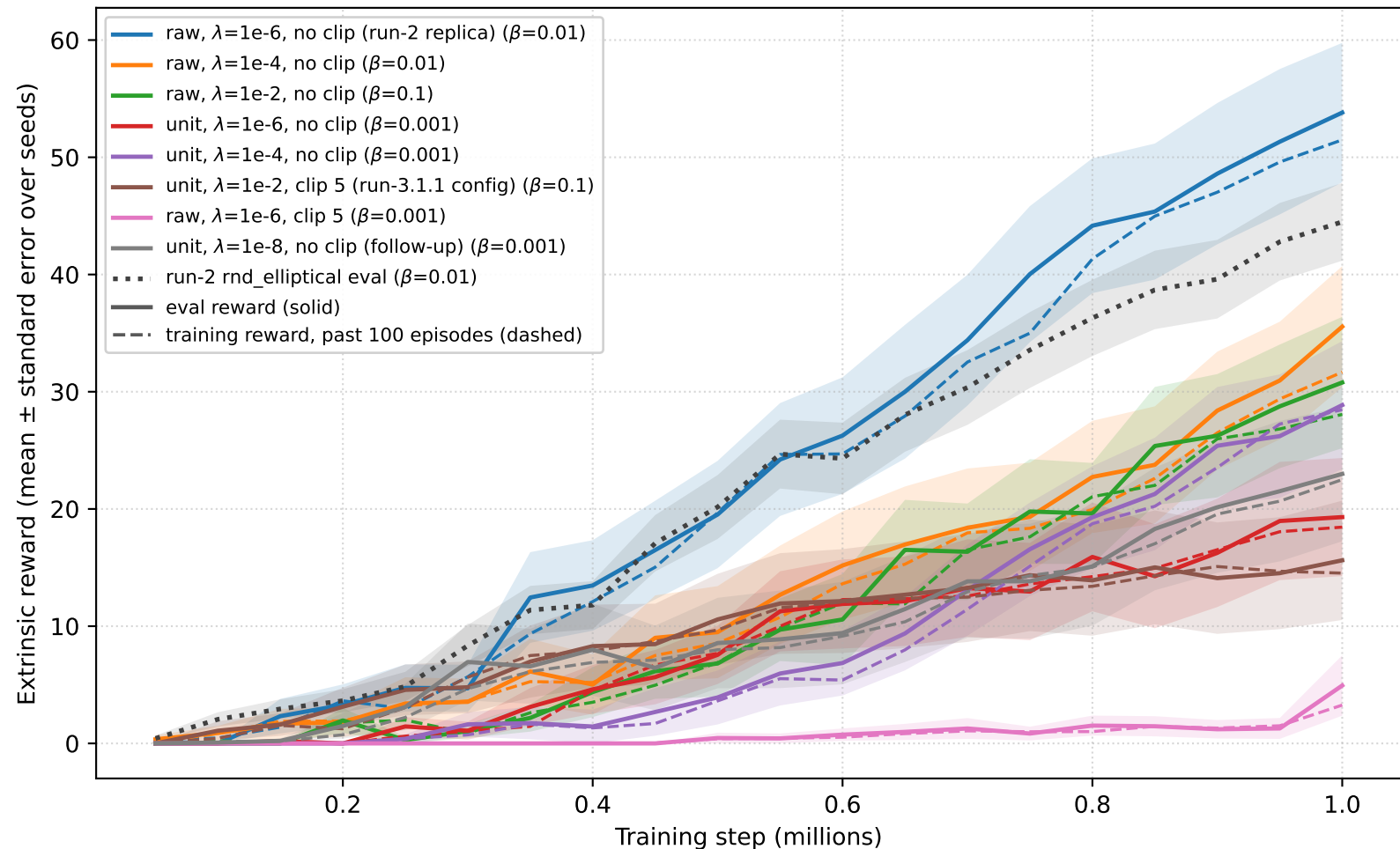
Train run 3.1.2: eval (solid) and training (dashed) reward, key cells at their best \beta
